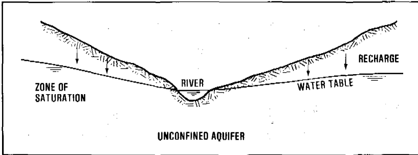
Figure 7.4a Infiltration of water into an unconfined aquifer during the wet season
