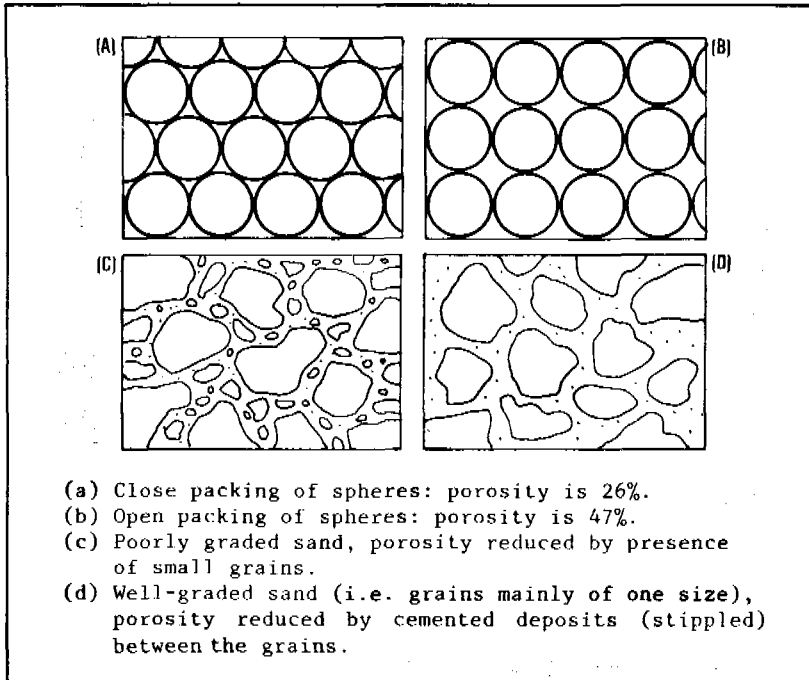
Figure 7.1. Porosity and texture
