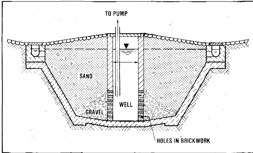
Figure 5.8. Venetian Cistern
