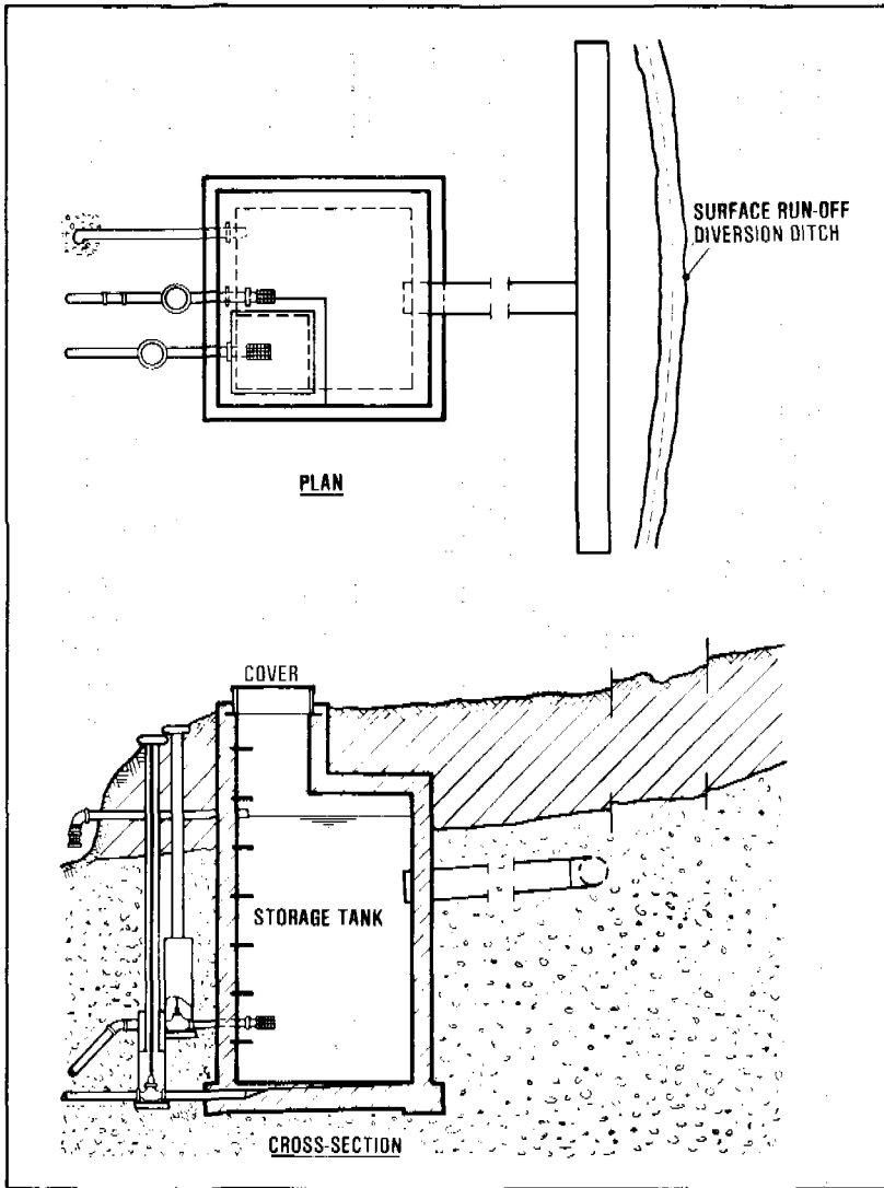
Figure 6.14. Artesian contact spring of large lateral width
