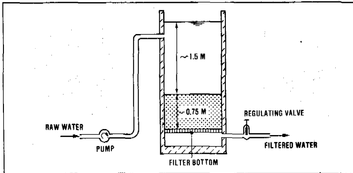
Figure 7 Experimental slow sand filter
