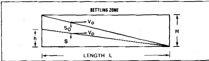
Figure 3 Particles travel path in the settling zone
