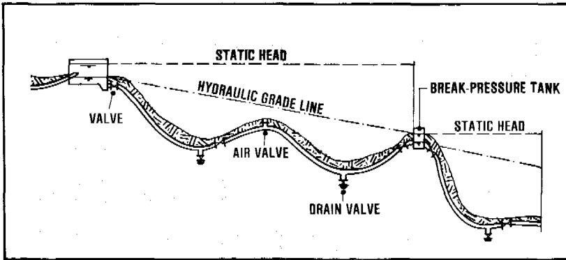
Figure 18.2. Pressure pipeline
