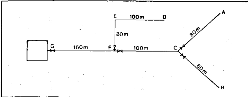
Figure 19.20. Simple water distribution system (schematic)
