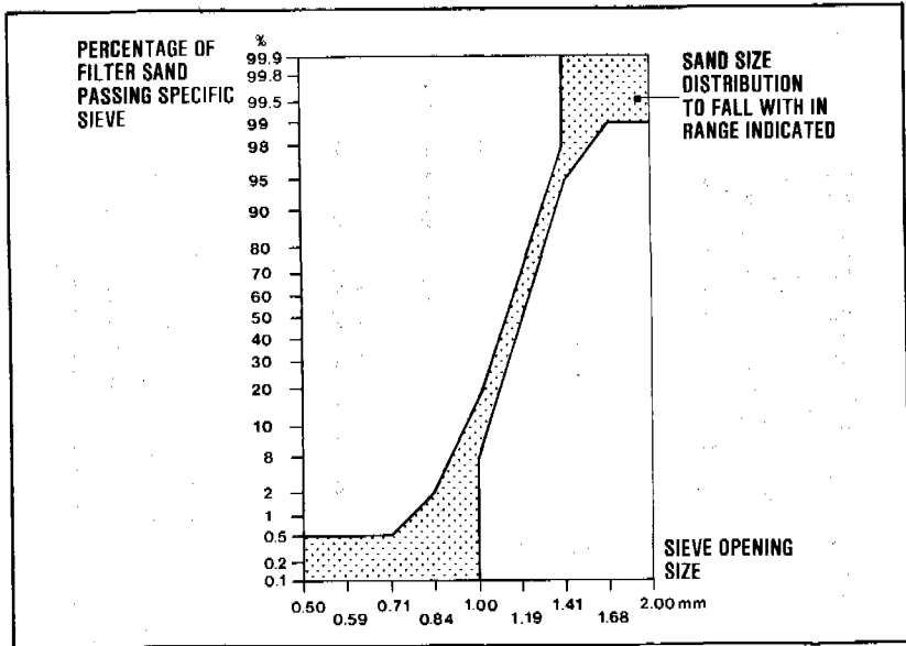
Figure 16.23. Specification of filter sand for pre-treatment of river water
