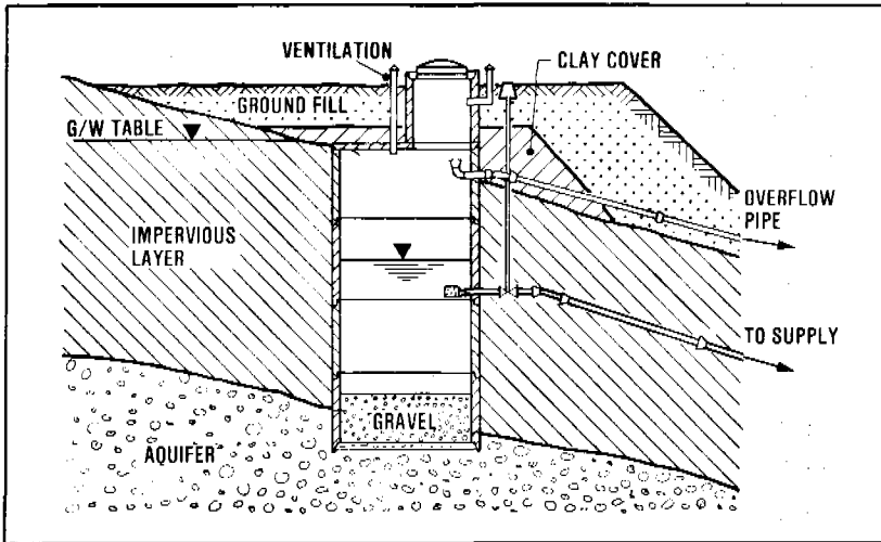
Figure 6.13. Fissure spring of large capacity
