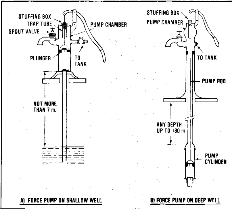
Figure 10.6. Force pumps
