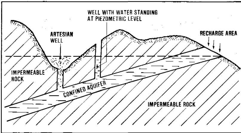
Figure 7.5. Confining aquifer fed from a recharge area
