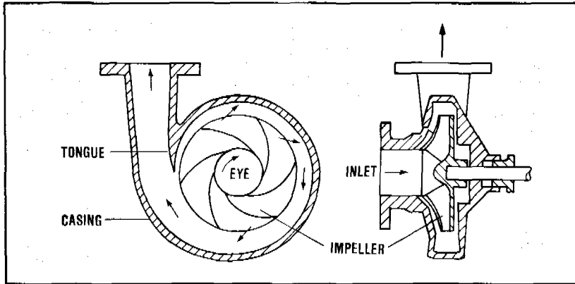
Figure 10.11. Centrifugal pump (Volute-type Casing)
