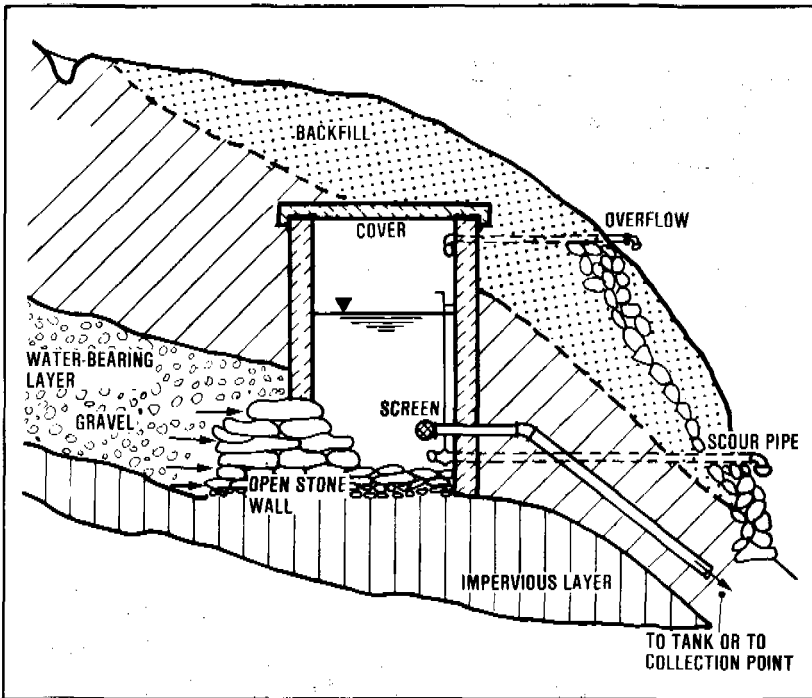
Figure 6.8. Spring water storage chamber ('spring box')
