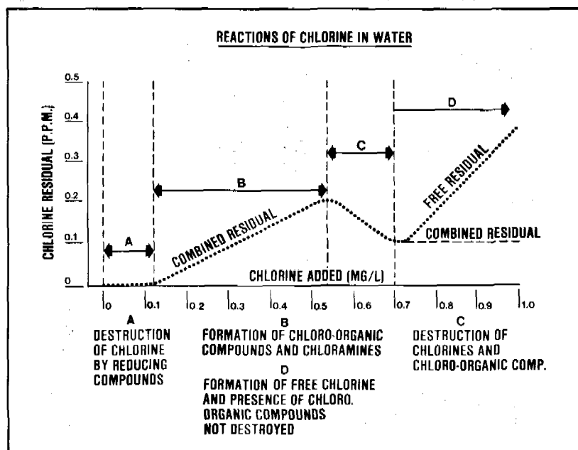
Figure 17.1. Reactions of chlorine in water
