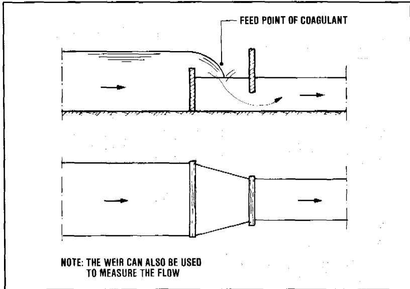
Figure 13.4. Overflow weir
