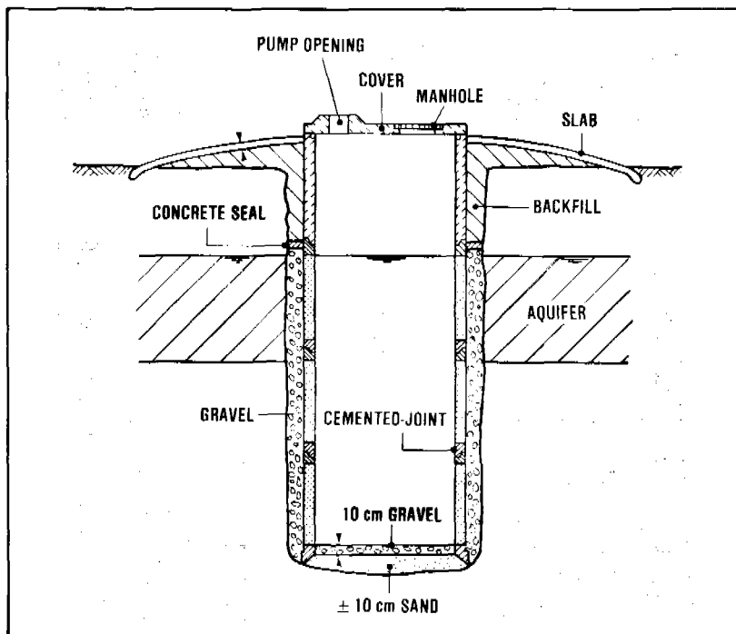
Figure 7.23. Dug well sealed for sanitary protection
