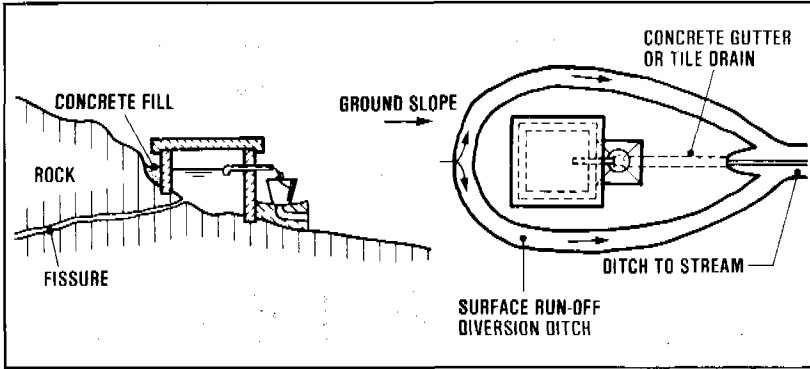
Figure 6.12. Fissure spring of small capacity
