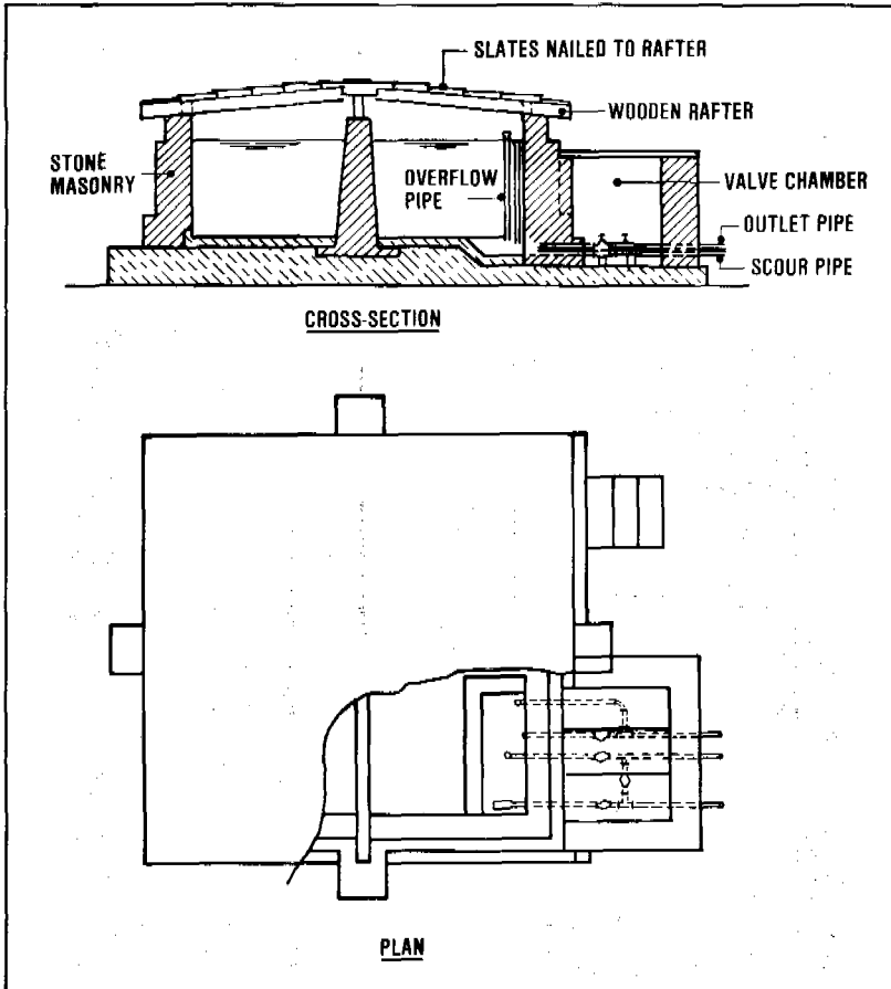
Figure 19.16. Small service reservoir
