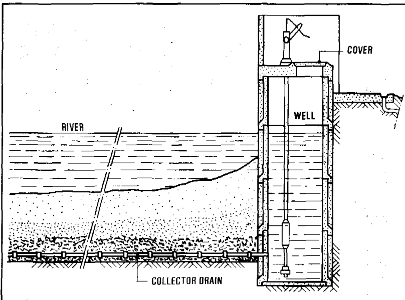
Figure 9.7. Horizontal collector drain under river bed
