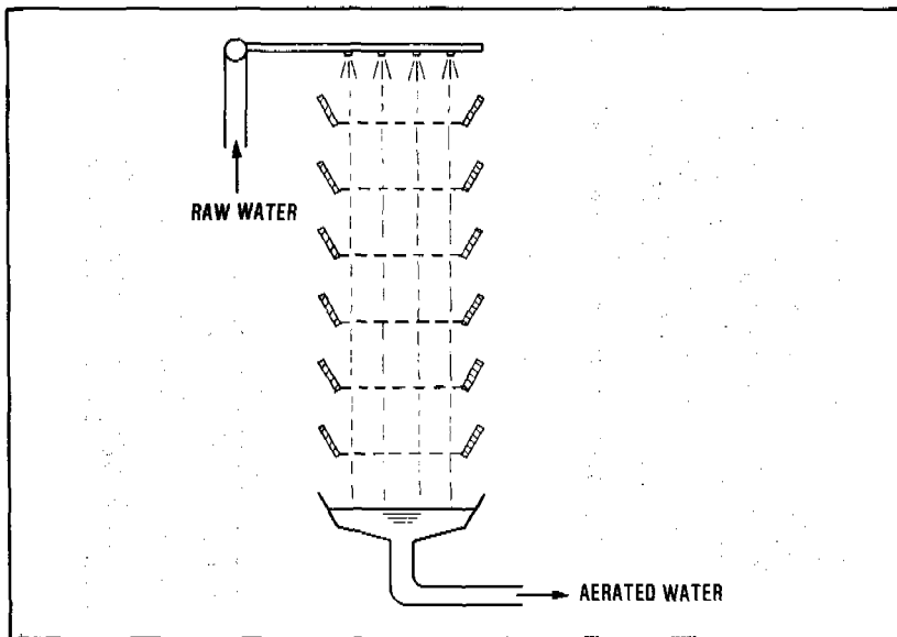
Figure 12.1. Multiple-tray aerator
