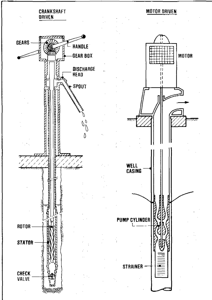
Figure 10.12. Shaft-driven pumps
