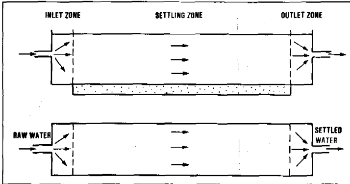
Figure 1 Schematic subdivision of settling tank
