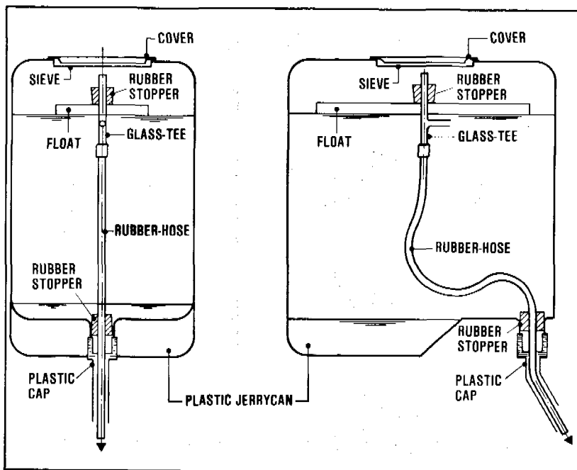
Figure 17.4. Equipment for feeding chlorine solution
