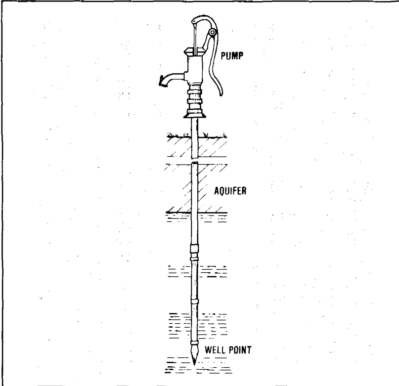
Figure 7.34. Driven well
