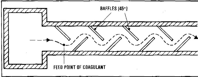
Figure 13.3. Baffled channel for rapid mixing
