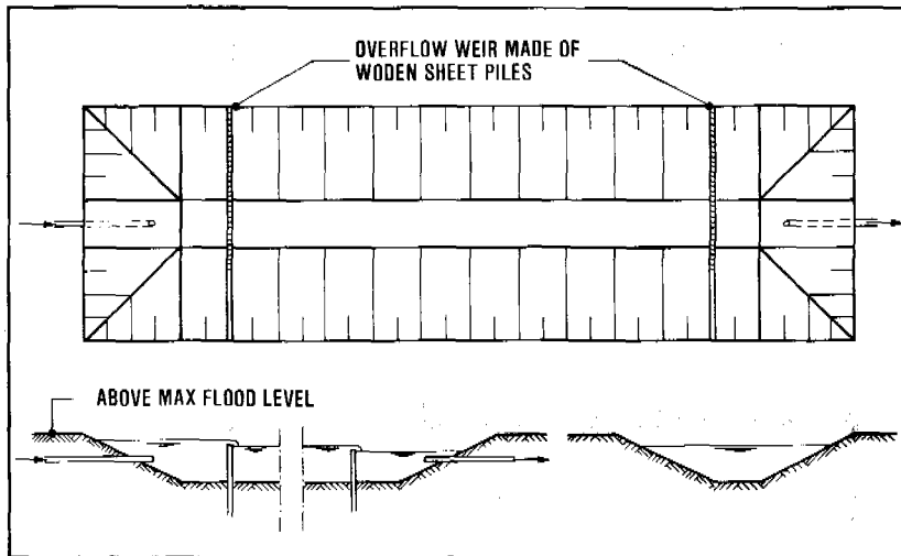
Figure 14.7. Dug basin as settling tank
