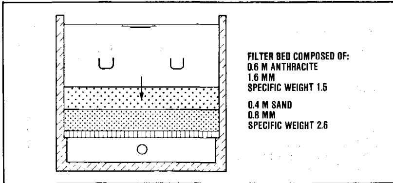
Figure 16.7. Dual-media filter bed
