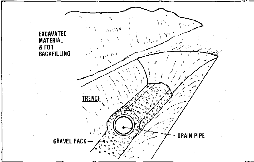
Figure 7.17. Drain construction
