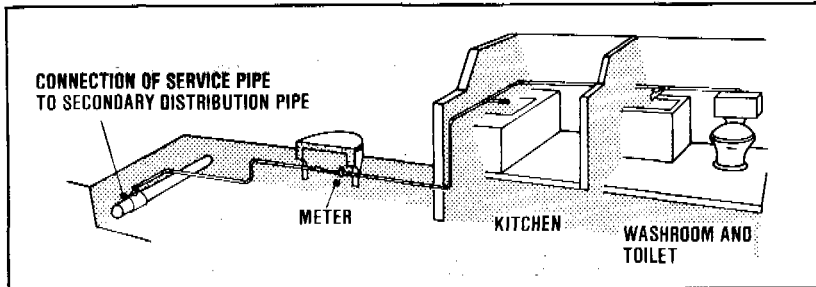
Figure 19.4. House connection
