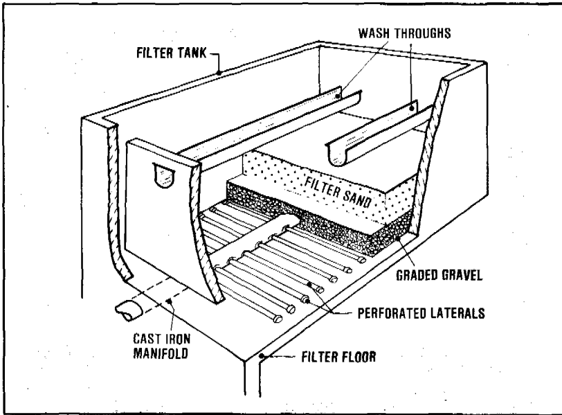
Figure 16.1. Rapid filter (open, gravity-type)
