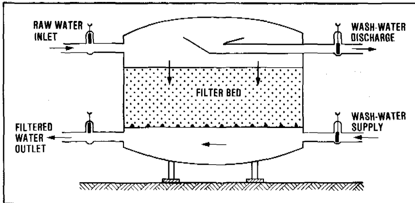
Figure 16.5. Pressure filter
