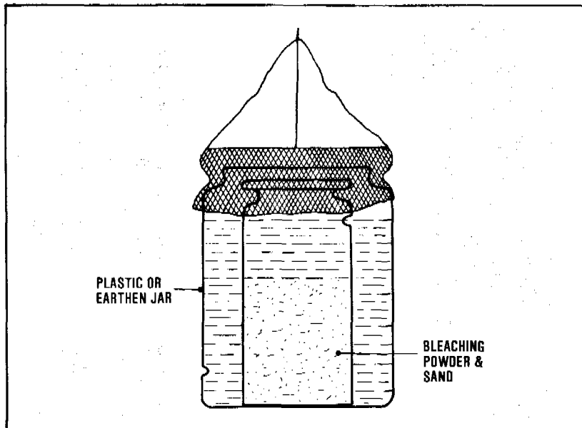
Figure 17.3. Double pot chlorinator
