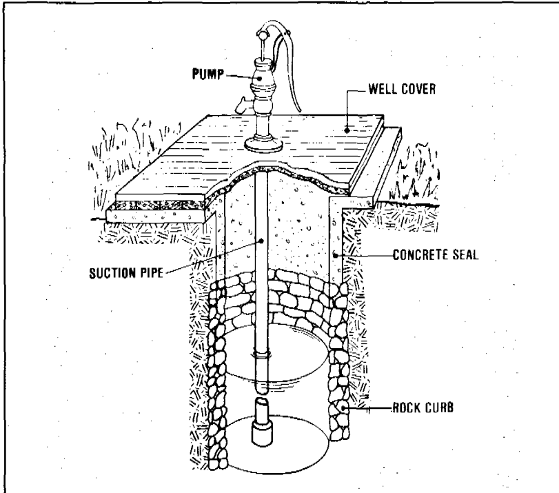
Figure 7.11. Dug well
