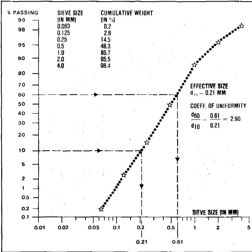
Figure 15.5. Grain size distribution of filter sand
