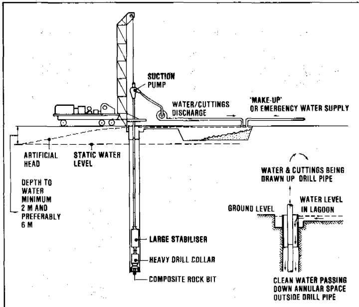
Figure 4 Reverse circulation rotary drill
