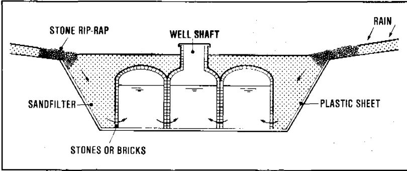
Figure 5.6. Cistern built of polythene tubes
