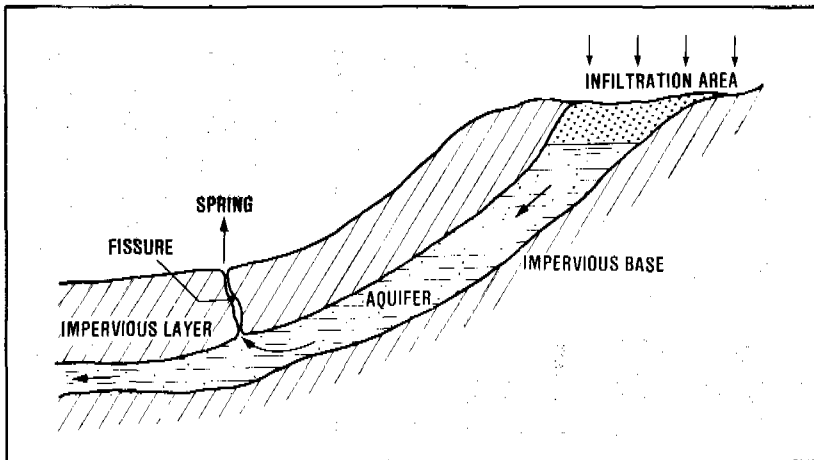
Figure 6.5. Artesian fissure spring
