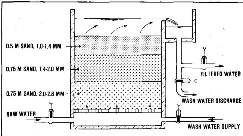
Figure 16.6. Upflow filter
