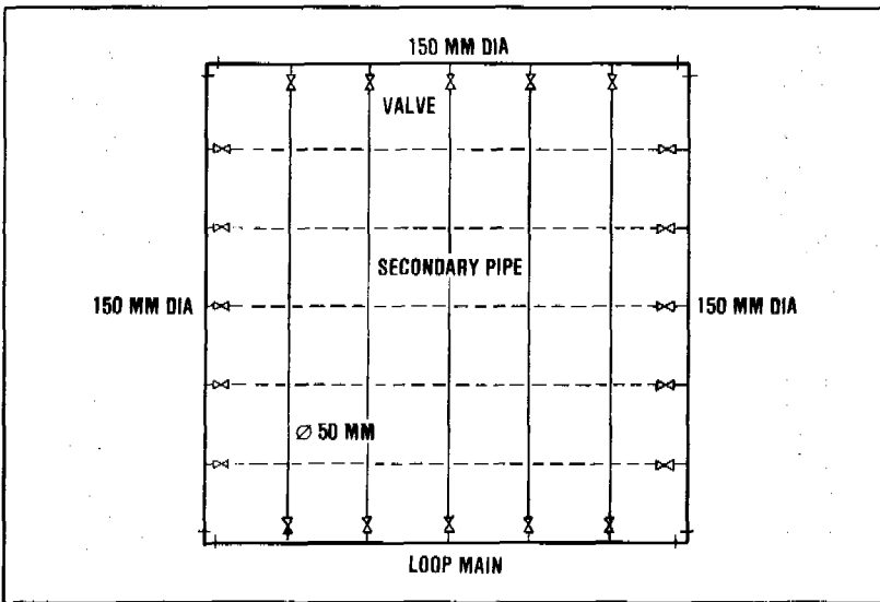
Figure 19.3. Over-crossing single pipes
