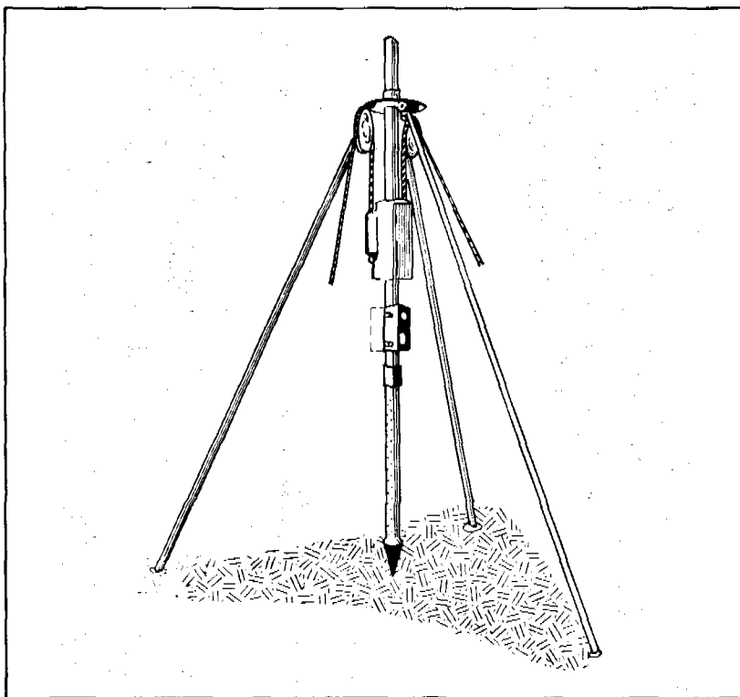
Figure 7.35. Well driving arrangement
