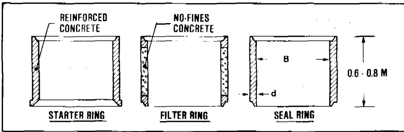
Figure 7.29. Pre-fabricated concrete rings
