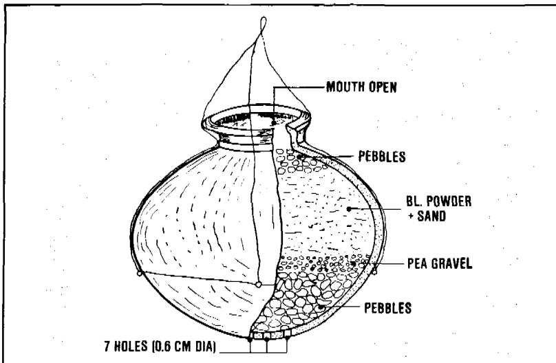
Figure 17.2. Chlorination pot with holes at the bottom
