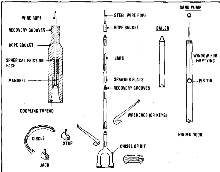
Figure 2 Percussion tools
