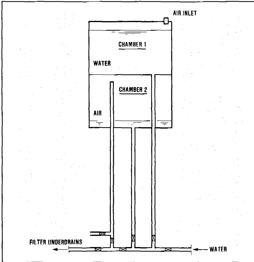
Figure 16.19 Air-and-water back-wash arrangement
