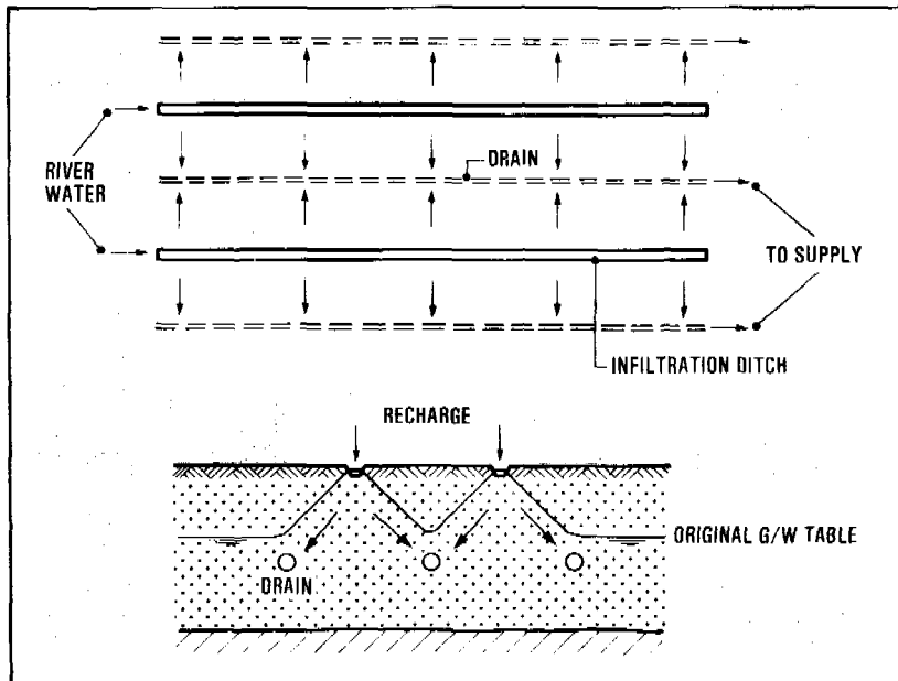
Figure 9.11. Water recharge in shallow aquifer using infiltration ditches and drains
