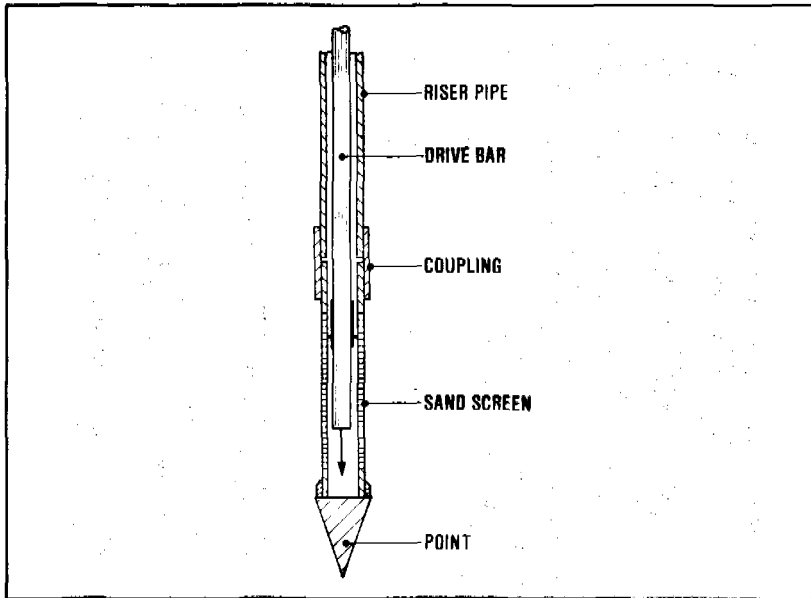
Figure 7.36. Well driving with inside drive bar
