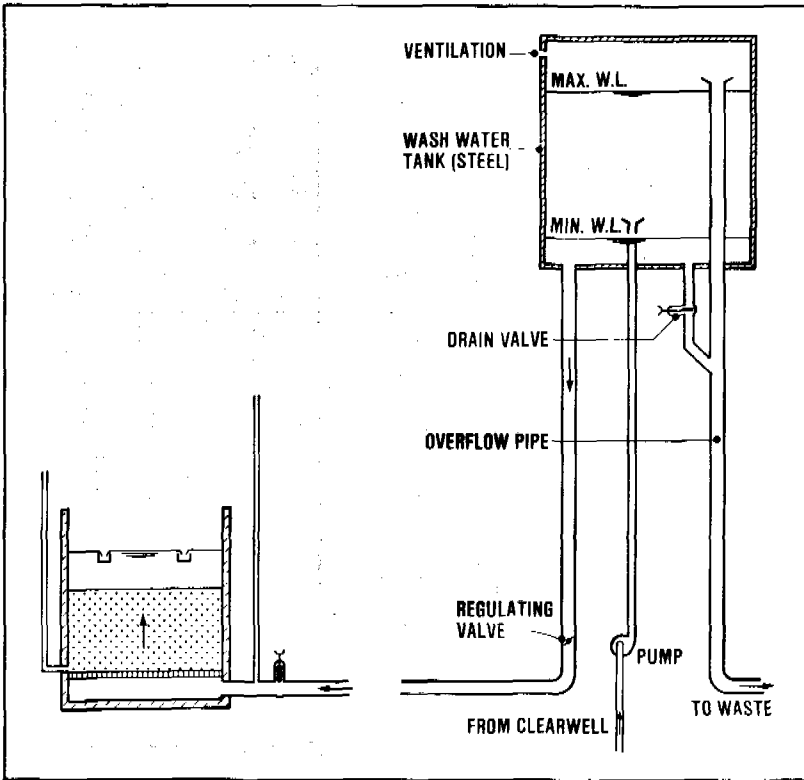
Figure 16.13. Wash-water tank arrangement
