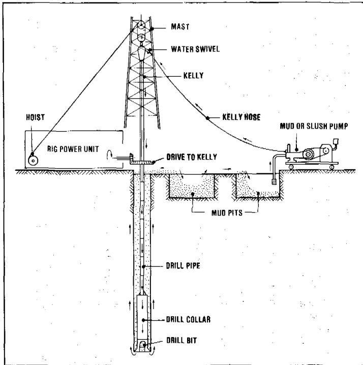
Figure 3 Normal direct circulation rotary drill
