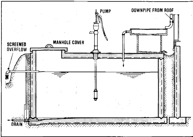
Figure 5.7. Rainwater storage arrangement
