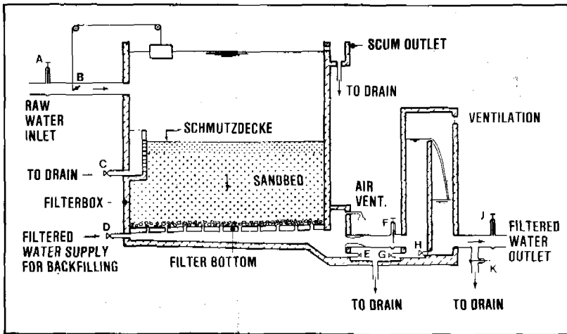
Figure 15.3. Slow sand filter
