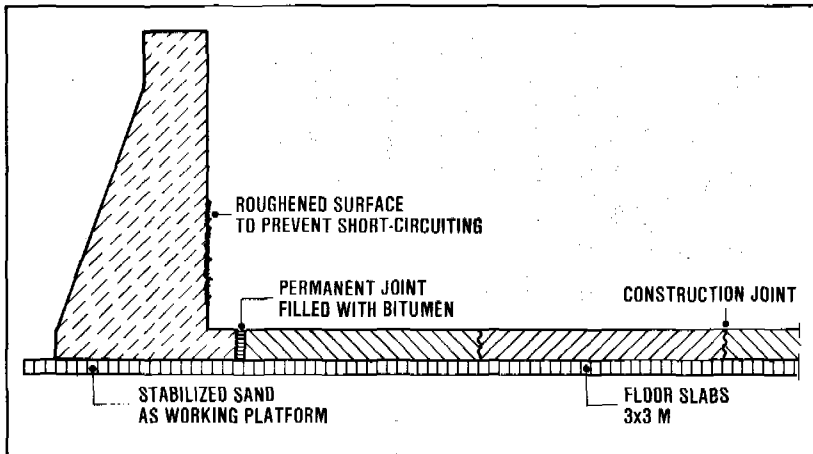
Figure 15.6. Slow sand filter constructed in mass concrete
