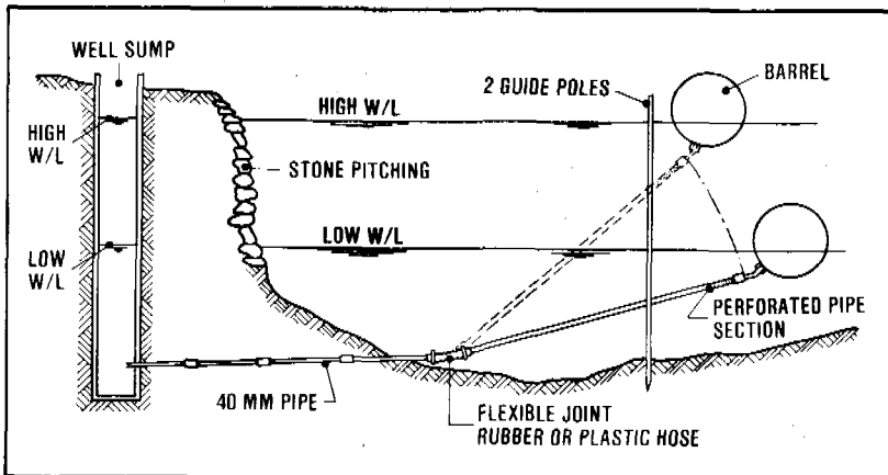
Figure 8.9. Float intake
