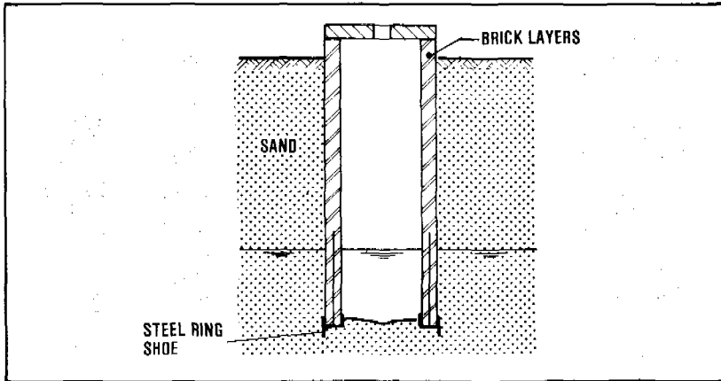
Figure 7.27. Dug well with brickwork lining.
