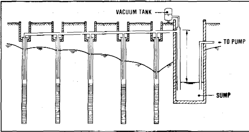
Figure 7.13. Battery of tubewells
