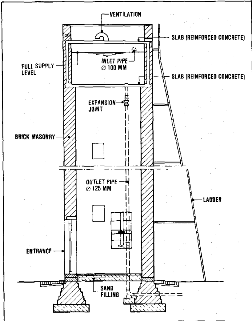
Figure 19.17. Elevated service reservoir
