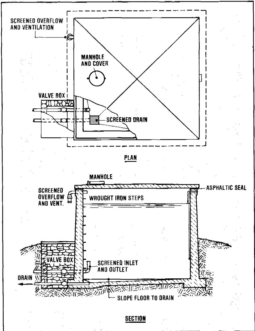
Figure 19.15. Construction details of small reservoir
