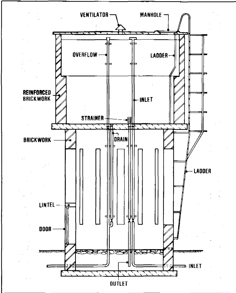
Figure 19.18. Elevated service reservoir
