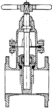
GATE VALVE
