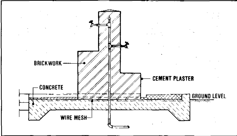
Figure 19.7. Cross-section of multiple-tap standpipe
