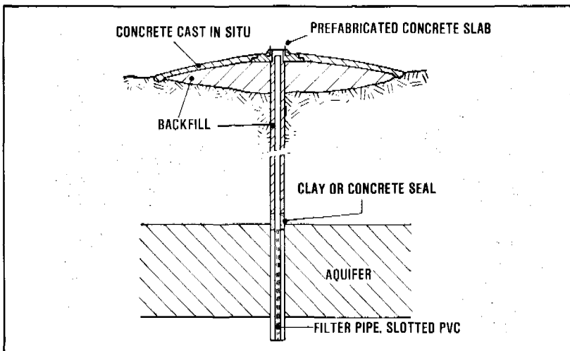
Figure 7.12. Tube well
