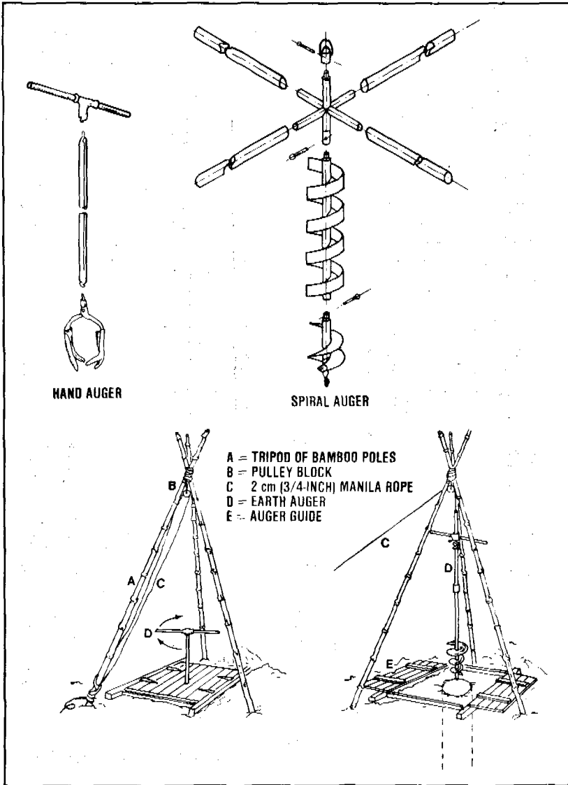
Figure 7.38 Well boring equipment
