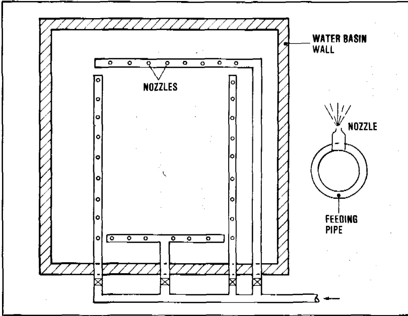
Figure 12.7. Nozzled spray aerator
