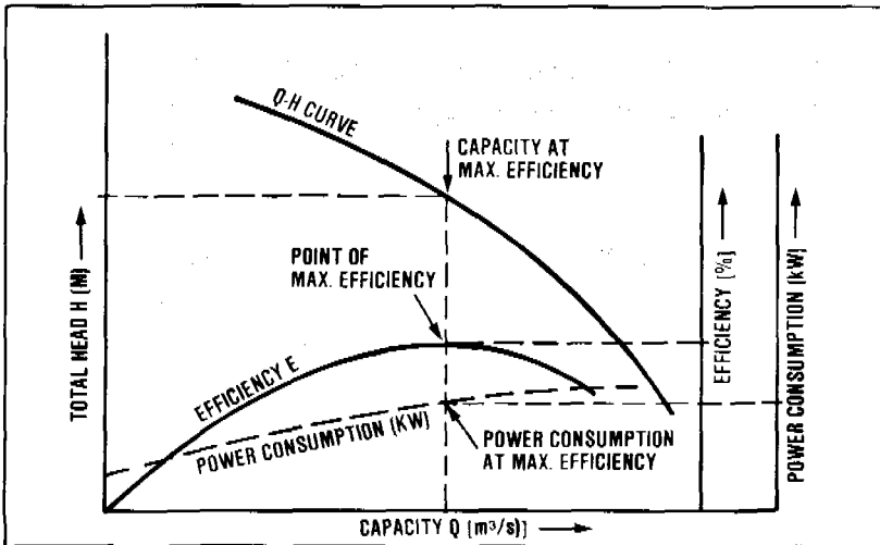
Figure 18.11. Typical pump characteristic curve
