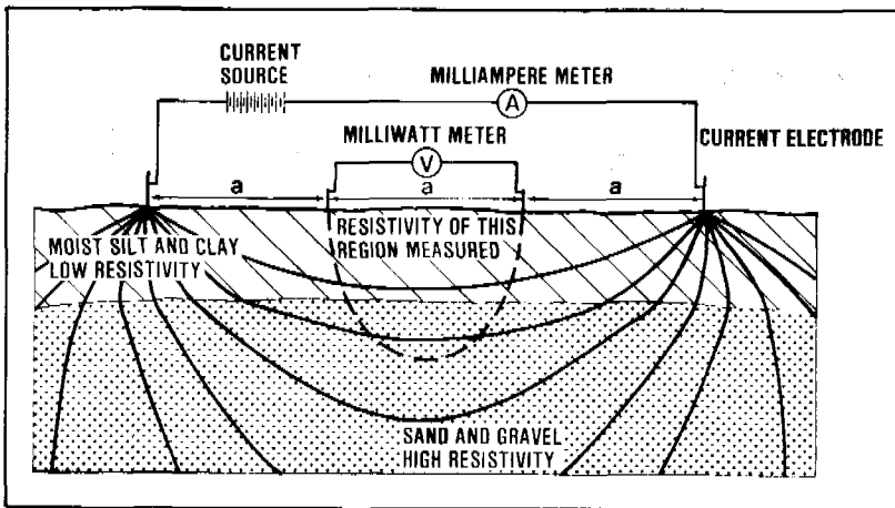
Figure 7.7. Electrical resistivity measuring arrangement
