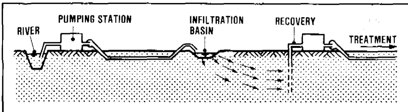
Figure 9.10. Scheme for artificial recharge and recovery
