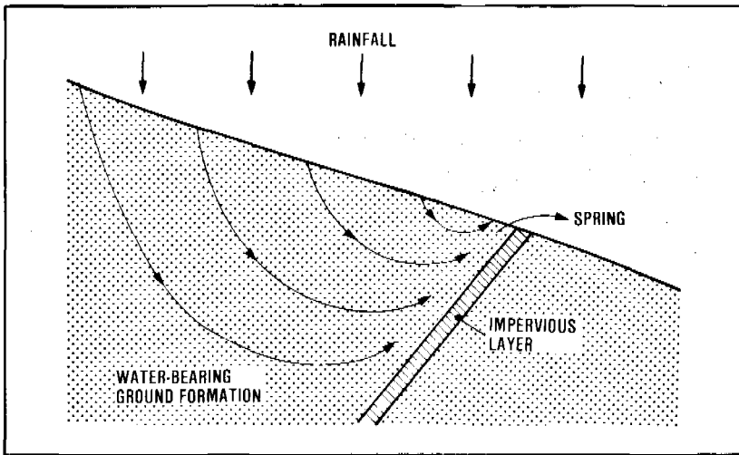
Figure 6.3. Gravity overflow spring
