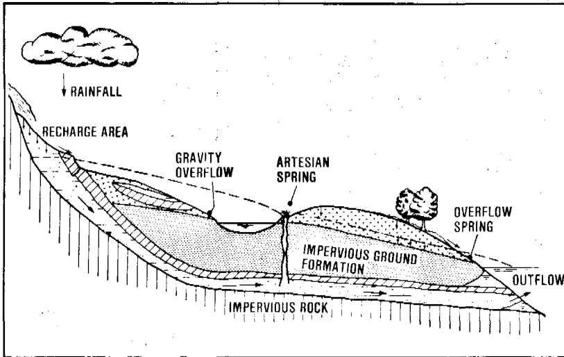
Figure 6.1. Occurrence of springs
