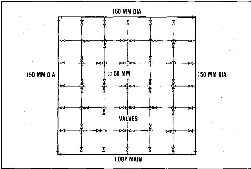
Figure 19.2. Fully-interconnected pipes.
