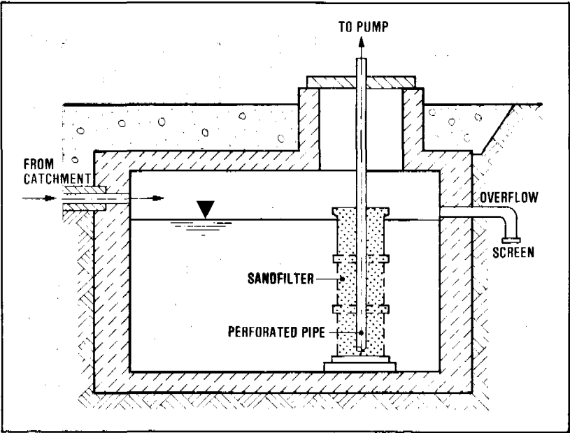
Figure 5.9. Withdrawal of filtered rainwater from storage
