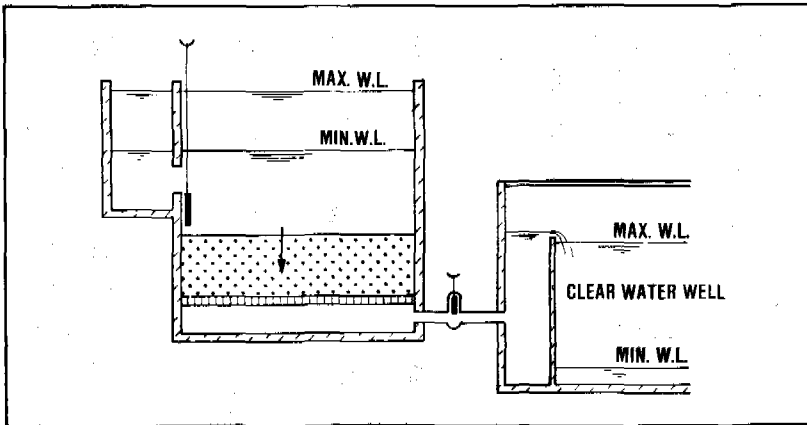
Figure 16.11. Declining-rate filtration
