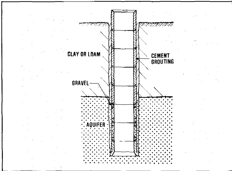
Figure 7.28. Dug well construction with pre-fabricated rings.
