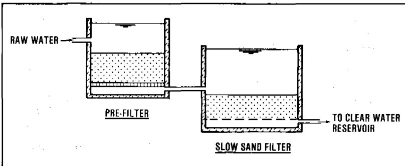
Figure 16.3. Rapid filtration-followed by slow sand filtration
