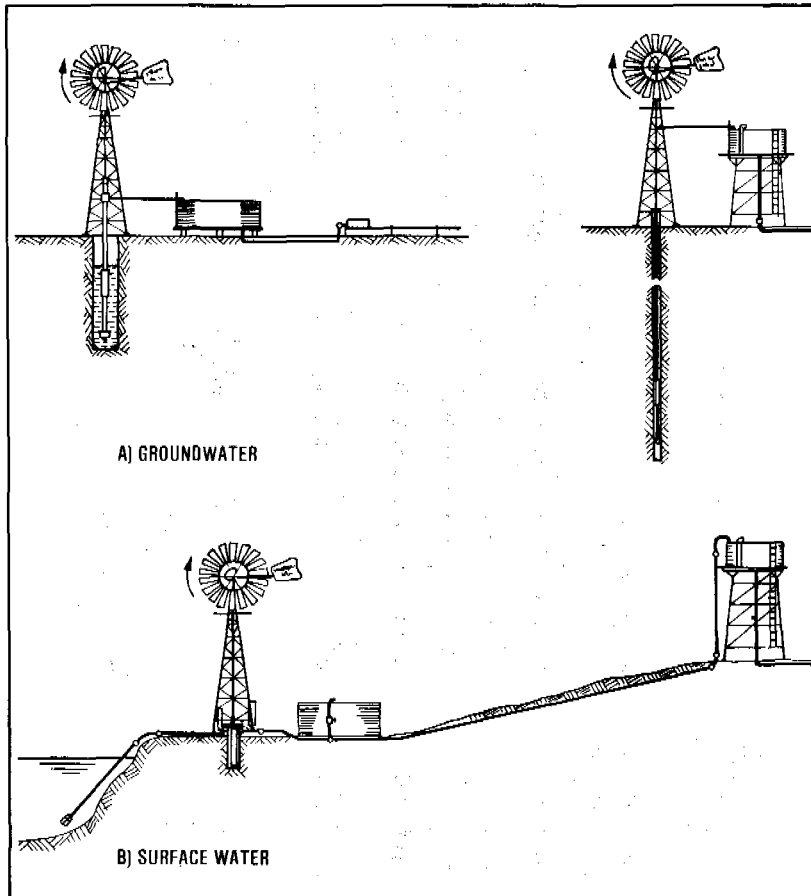
Figure 10.2. Windmill-pumped water supply systems
