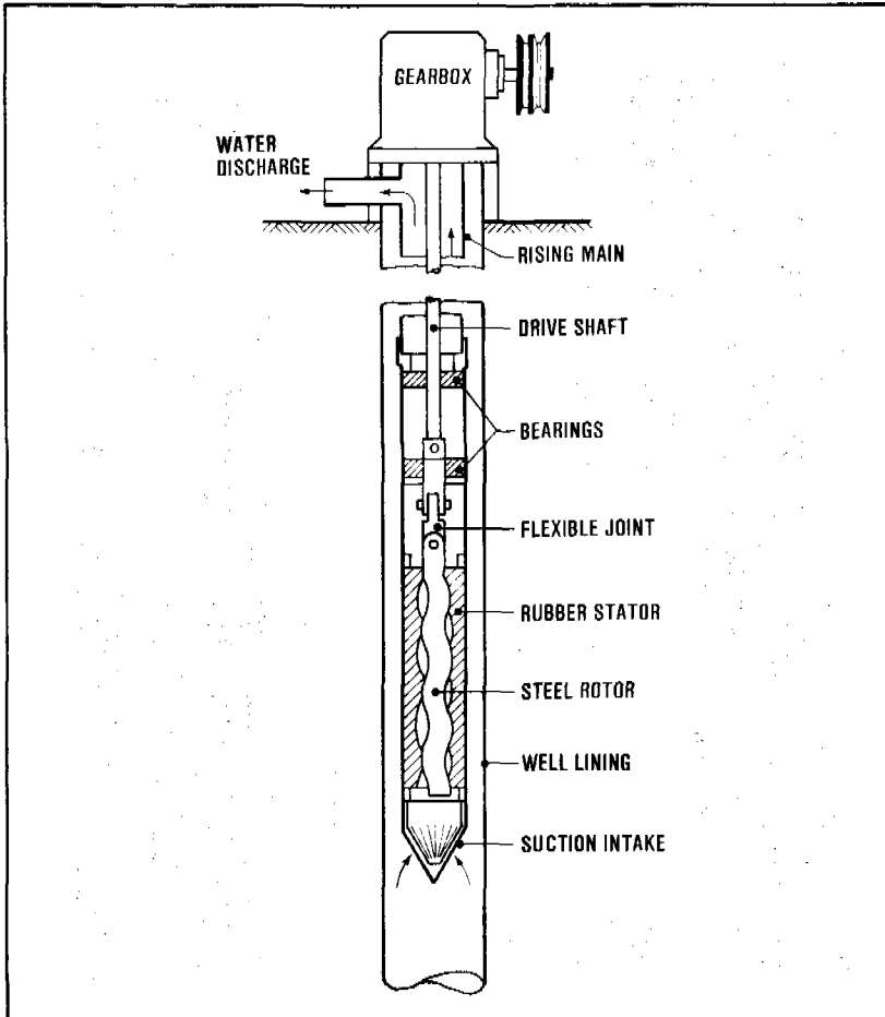
Figure 10.9. Helical rotor pump
