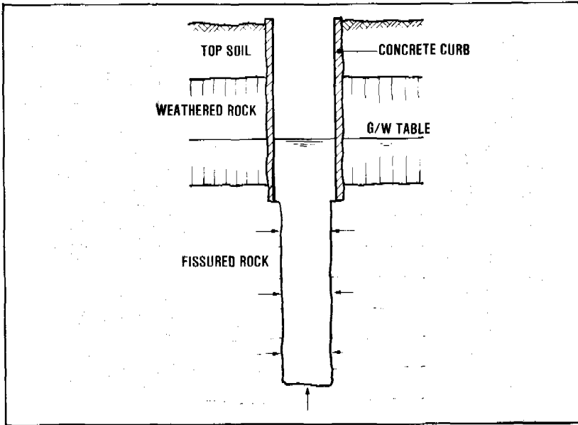
Figure 7.19. Dug well in rock formation
