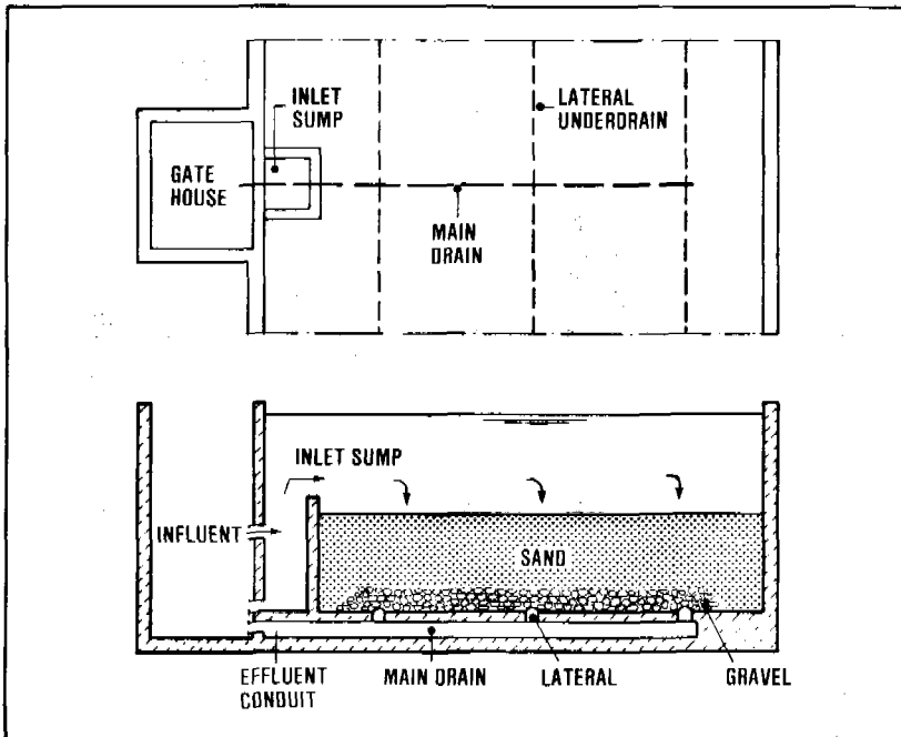
Figure 15.1. Slow sand filter
