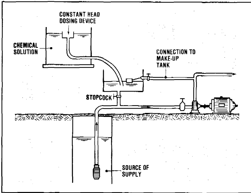
Figure 17.6. Chlorination arrangement for pumped supplies
