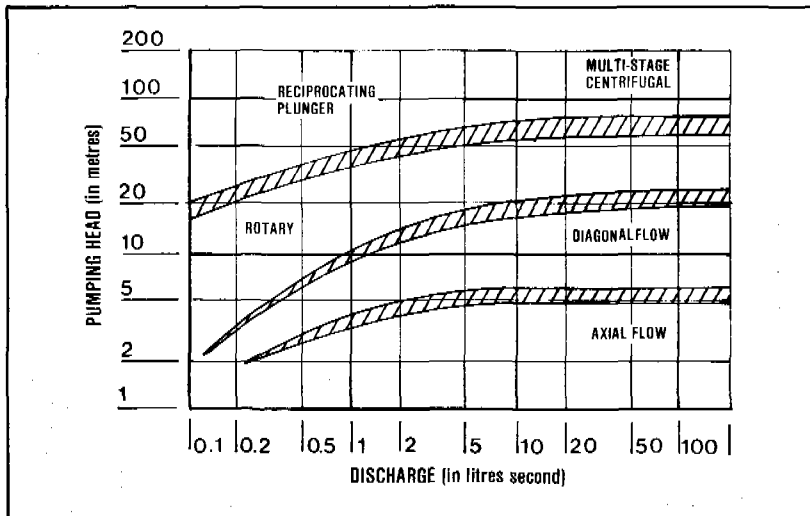
Figure 10.3. Pump type selection chart
