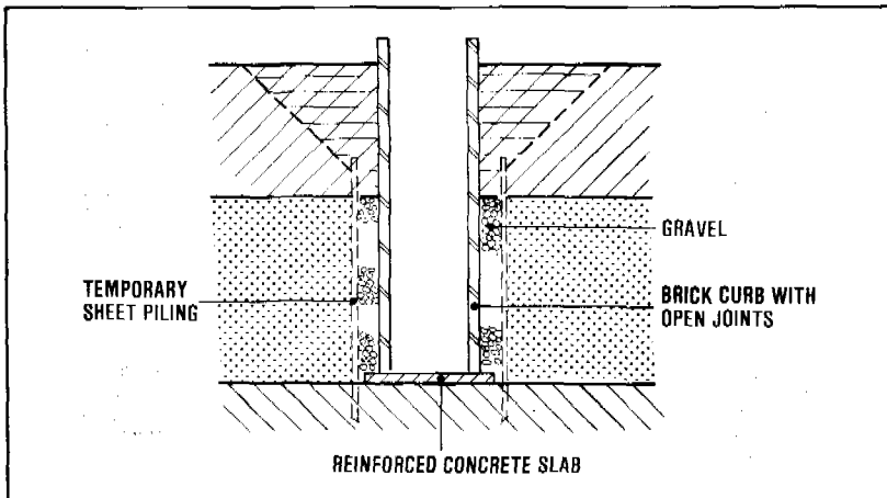
Figure 7.24. Dug well built in temporary excavation
