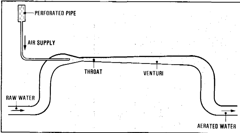
Figure 12.10. Venturi aerator
