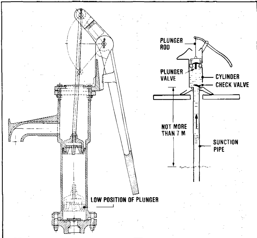
Figure 10.4. Suction pump (shallow well)
