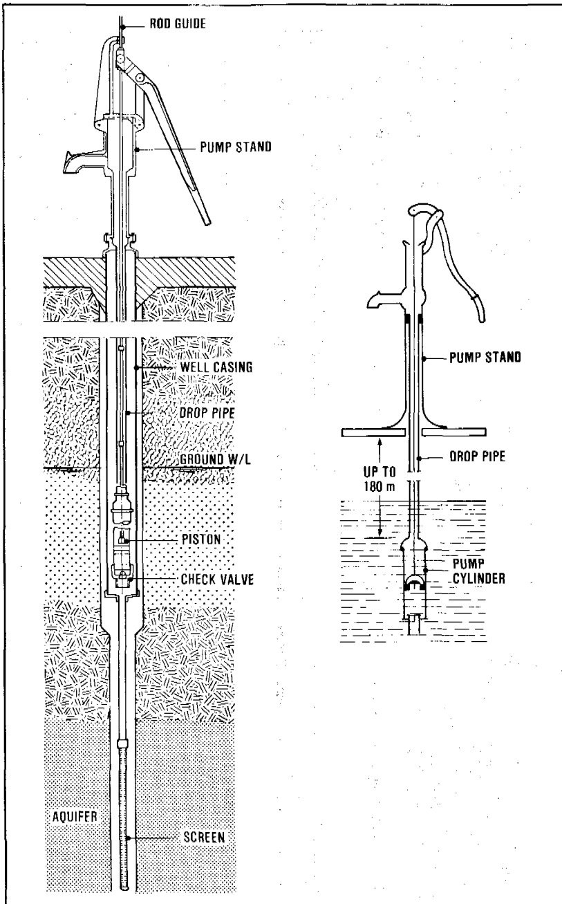
Figure 10.5. Lift pump (deep well)
