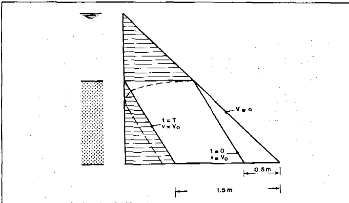
Figure 12 Pressure distribution in bed or rapid filter.
