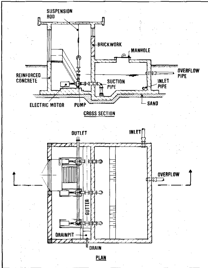
Figure 18.13. Pumping installation (dry pit)
