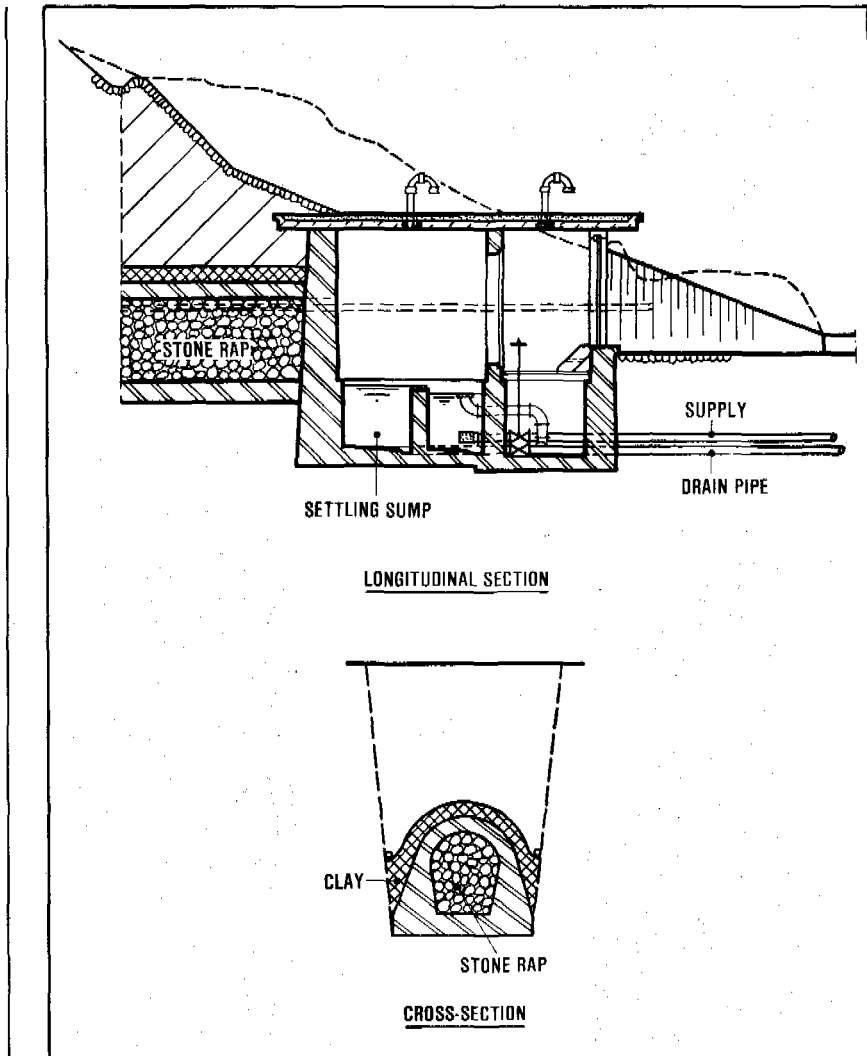
Fig. 6.15. Typical spring tapping structure
