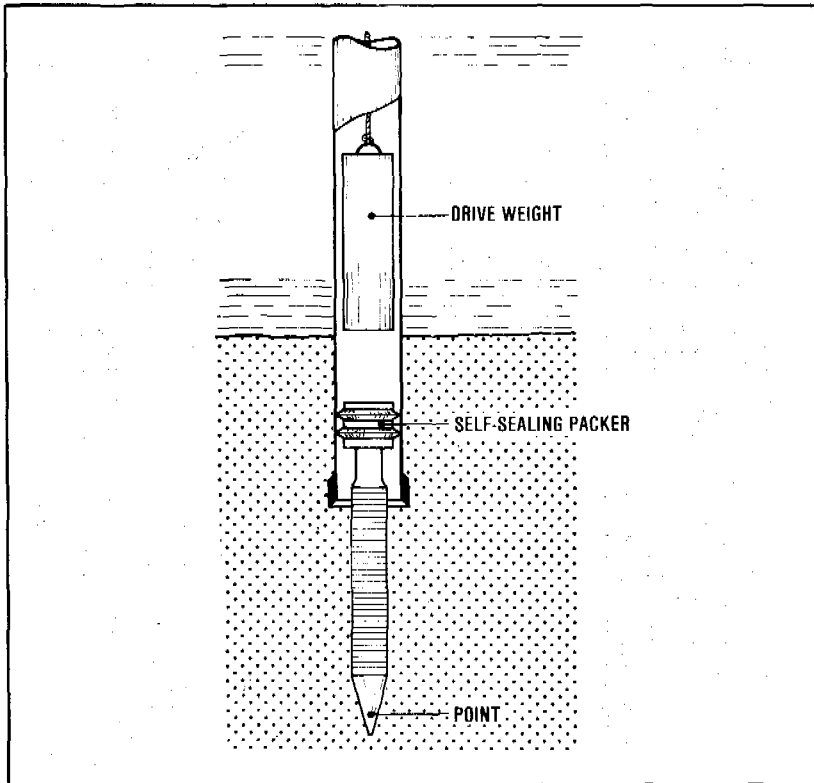
Figure 7.37. Well drive point with sliding joint
