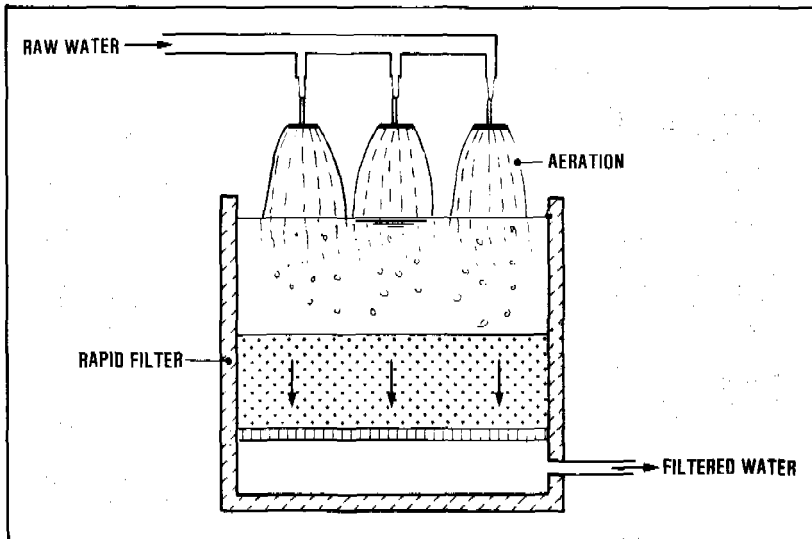
Figure 16.2. Rapid filtration of pre-treated (aerated) water
