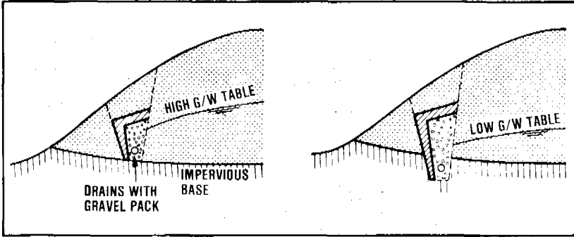
Figure 6.7. Tapping of a gravity spring
