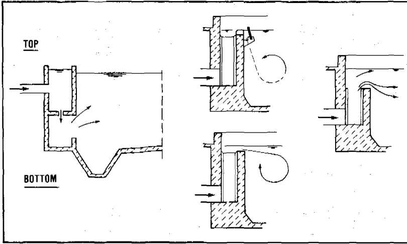
Figure 14.3. Inlet arrangements
