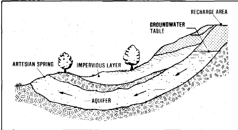
Figure 6.6. Artesian overflow spring
