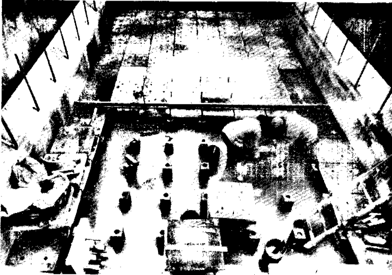
Figure 16.21. Underdrain system with false bottom and strainers
