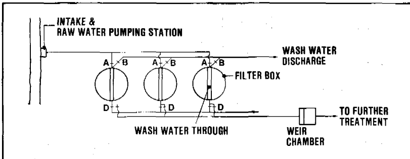
Figure 16.24. General layout of a rapid filtration plant
