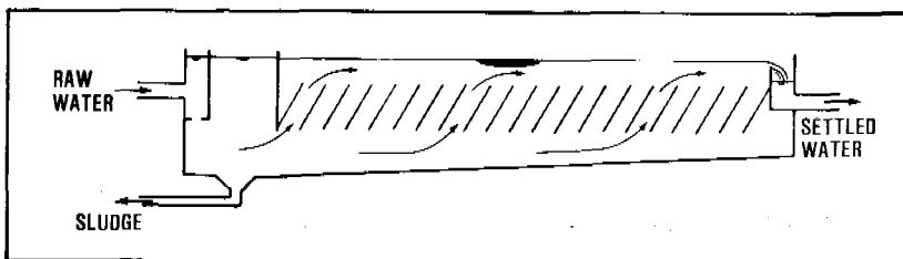
Figure 14.9. Tilted plate settling tank
