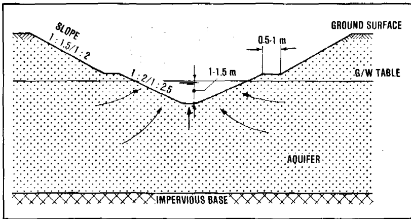
Figure 7.16. Design of seepage ditch
