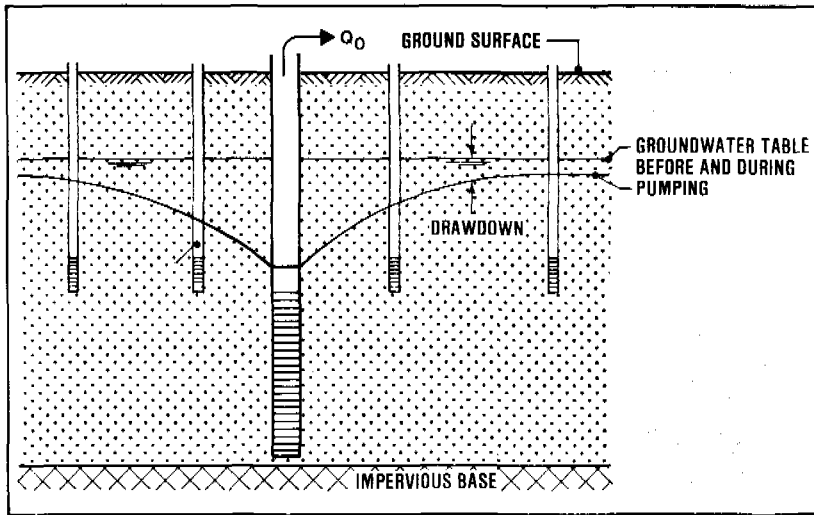
Figure 7.15. Test pumping
