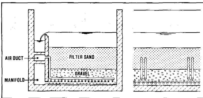
Figure 16.18. Backwashing with air and water
