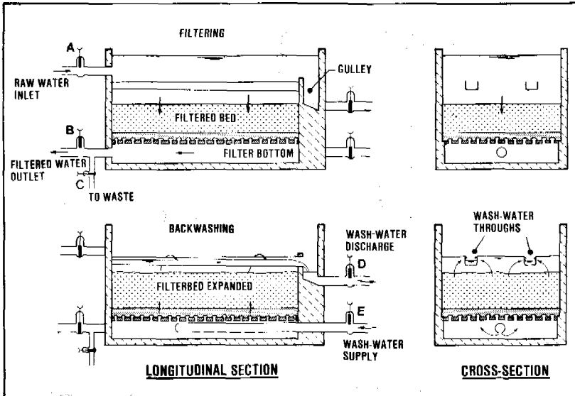
Figure 16.8. Rapid filter (gravity-type)
