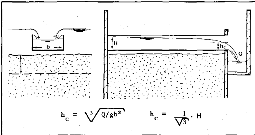
Figure 16.15. Flow condition in wash-water trough
