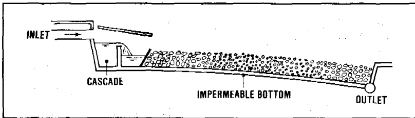
Figure 16.25. Horizontal gravel filter
