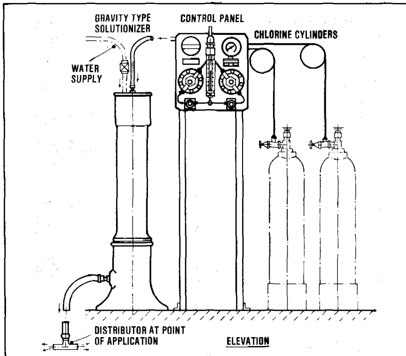
Figure 17.7. Chlorine gas apparatus with gravity-type solutionizer
