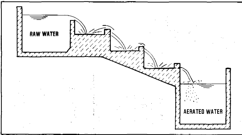
Figure 12.4. Cascade aerator
