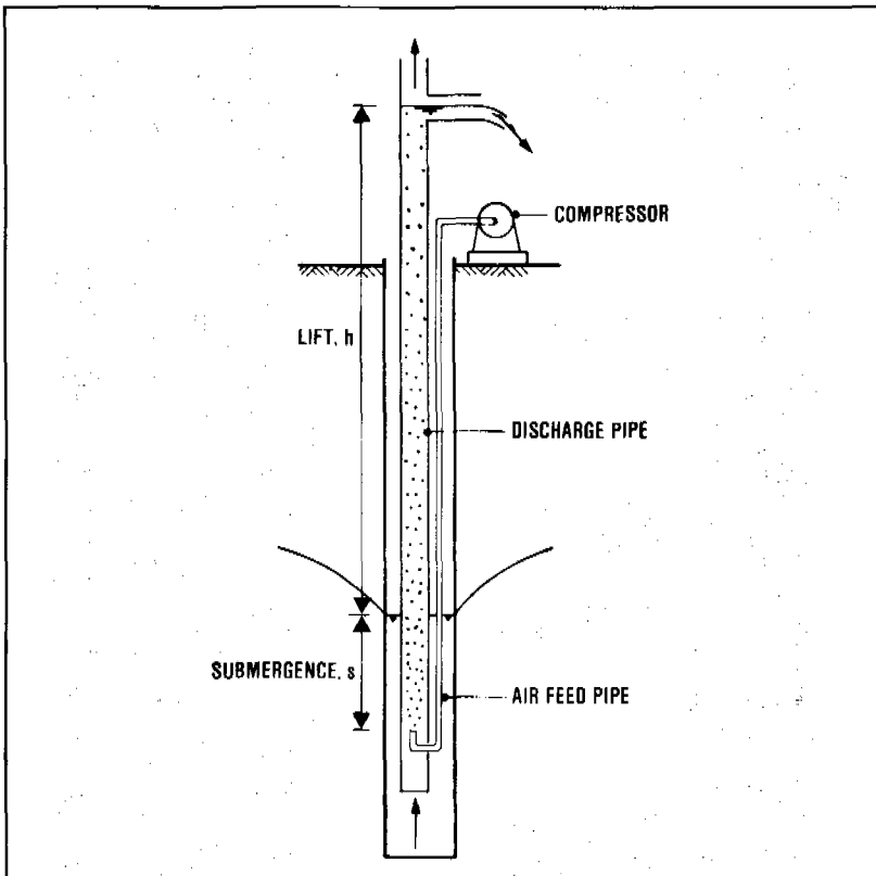
Figure 10.15. Air lift pump (schematic)
