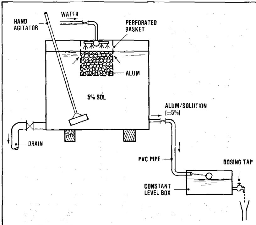
Figure 13.2. Chemical feed arrangement for alum
