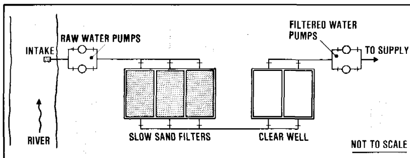
Figure 15.11. General arrangement for slow sand filtration plant
