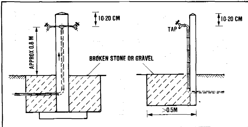
Figure 19.6. Cross-section of simple standpipes
