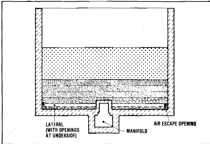
Figure 16.14. Lateral underdrain systems
