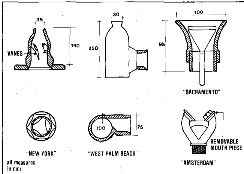
Figure 12.9. Nozzles for spray aerators
