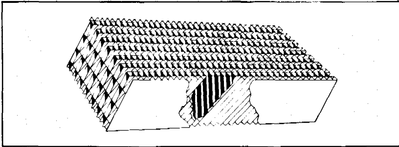
Figure 14.12. Module for tube settler
