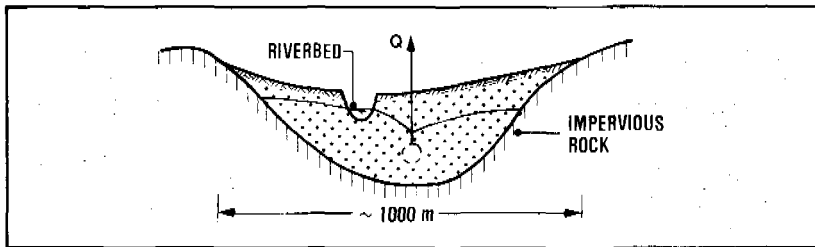
Figure 9.5. Induced recharge and groundwater recovery from an aquifer of small width
