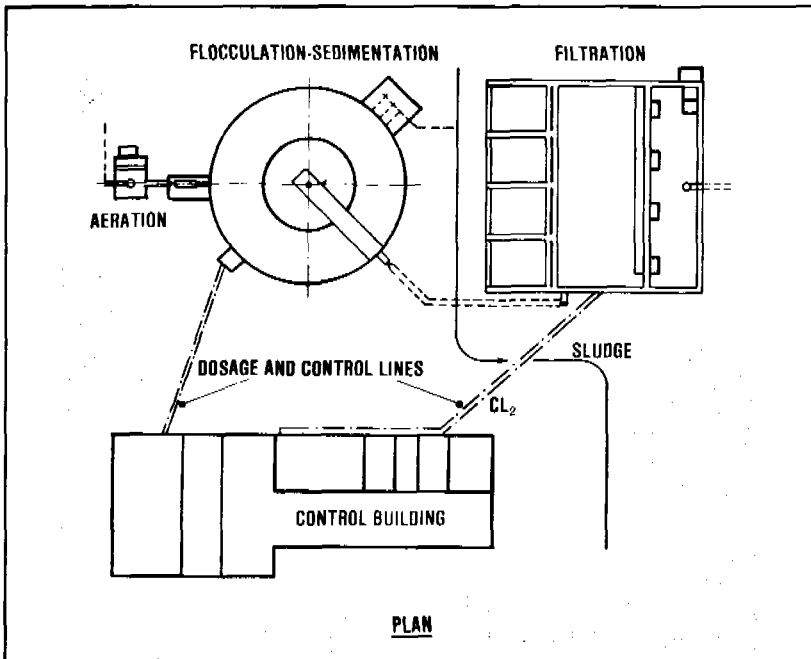
Figure 16.20. Rapid filtration plant layout
