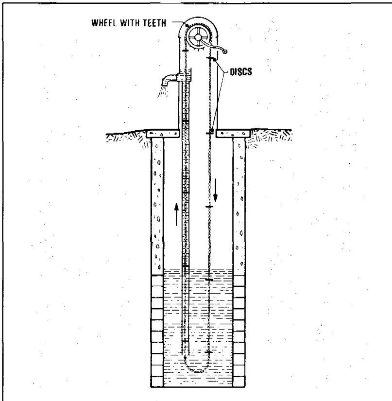
Figure 10.8. Chain pump
