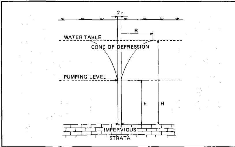
Figure 1. Water well pumping.
