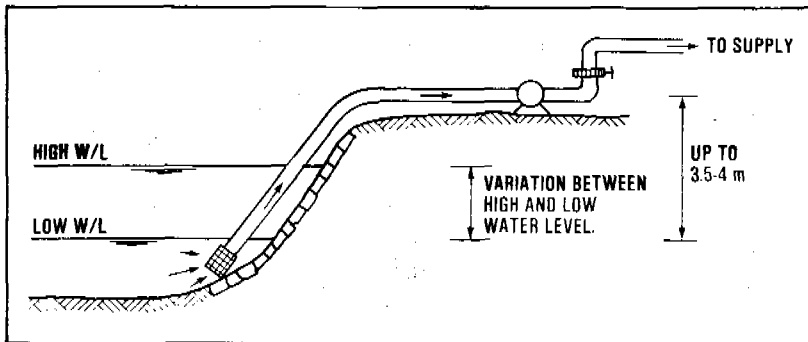
Figure 8.3. Pumped river water intake
