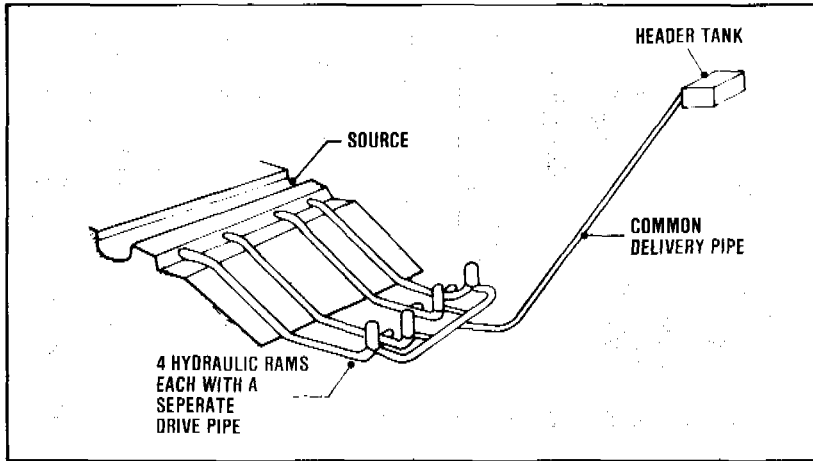
Figure 10.17. Hydraulic rams placed parallel
