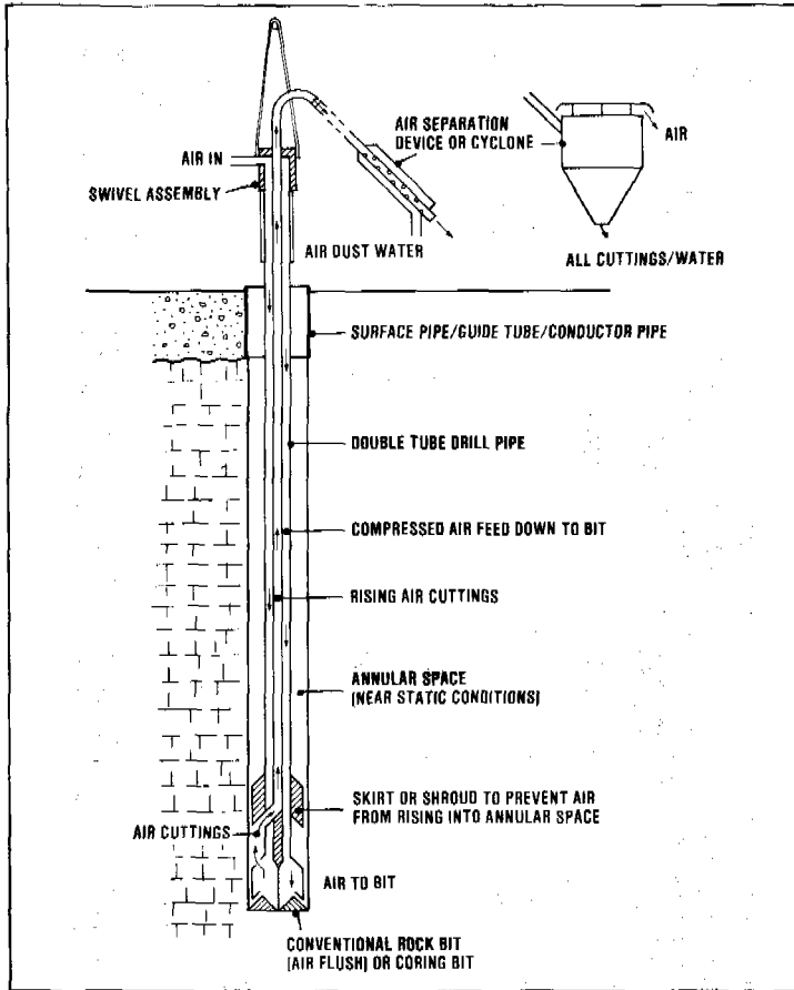
Figure 5 Reverse circulation air drilling
