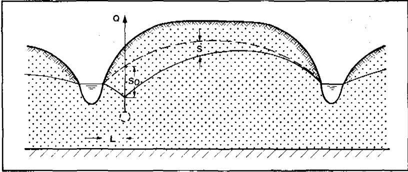
Figure 9.4. Induced recharge
