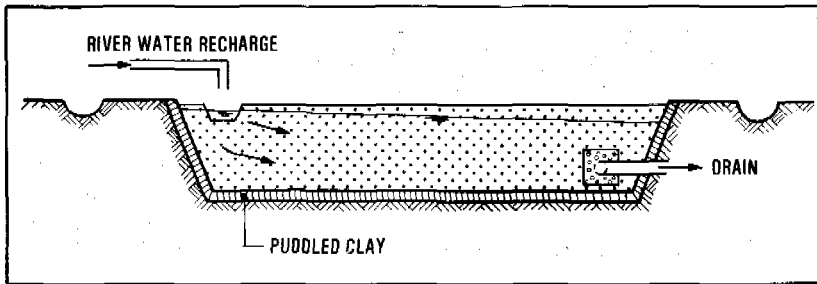
Figure 9.13. Small-capacity recharge scheme
