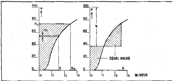
Figure 5 Cumulative frequency distribution of settling velocities
