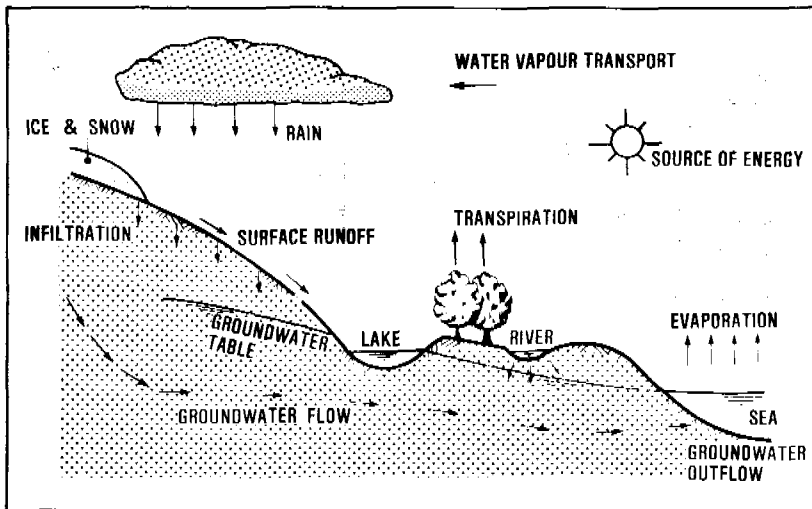
Figure 4.1. Hydrological cycle
