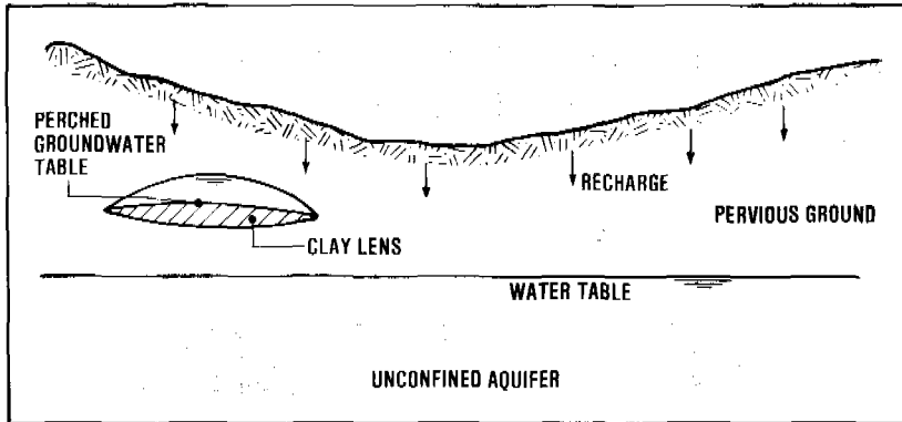
Figure 7.6. Perched water table
