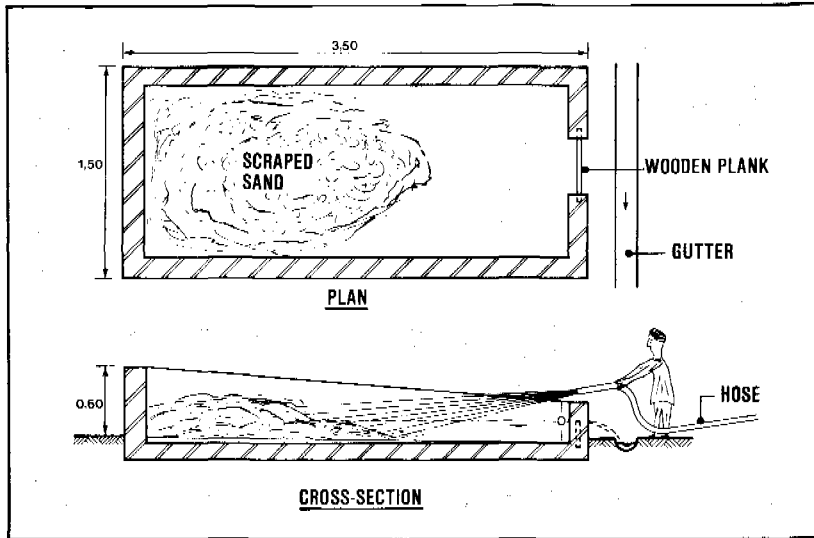
Figure 15.14. Sand washing platform
