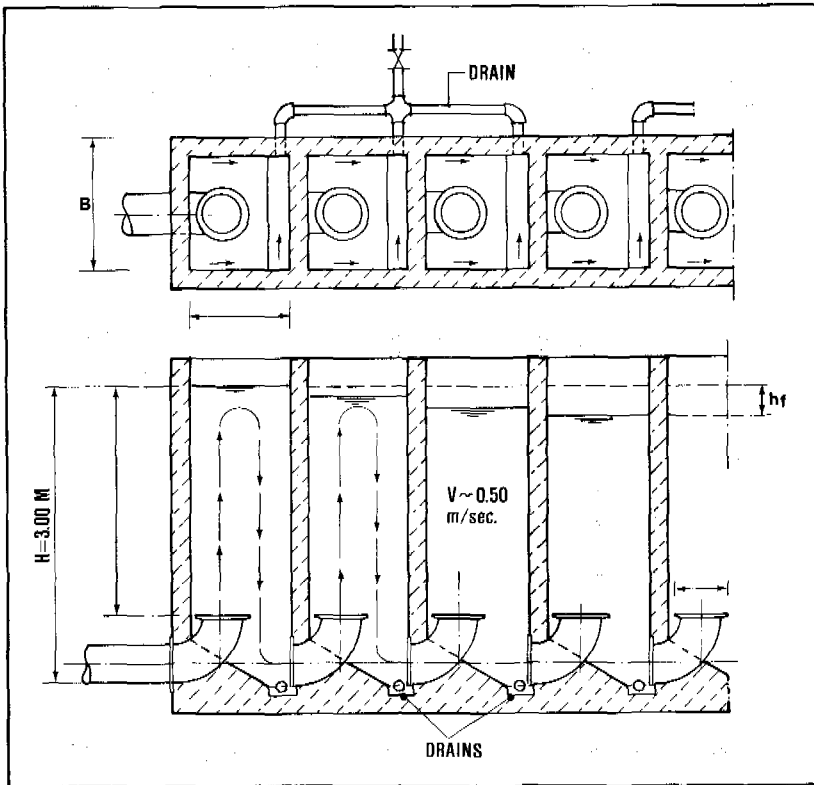
Fig. 13.10. 'Alabama'-type flocculator
