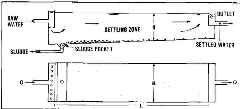
Figure 14.1. Rectangular horizontal flow settling tank
