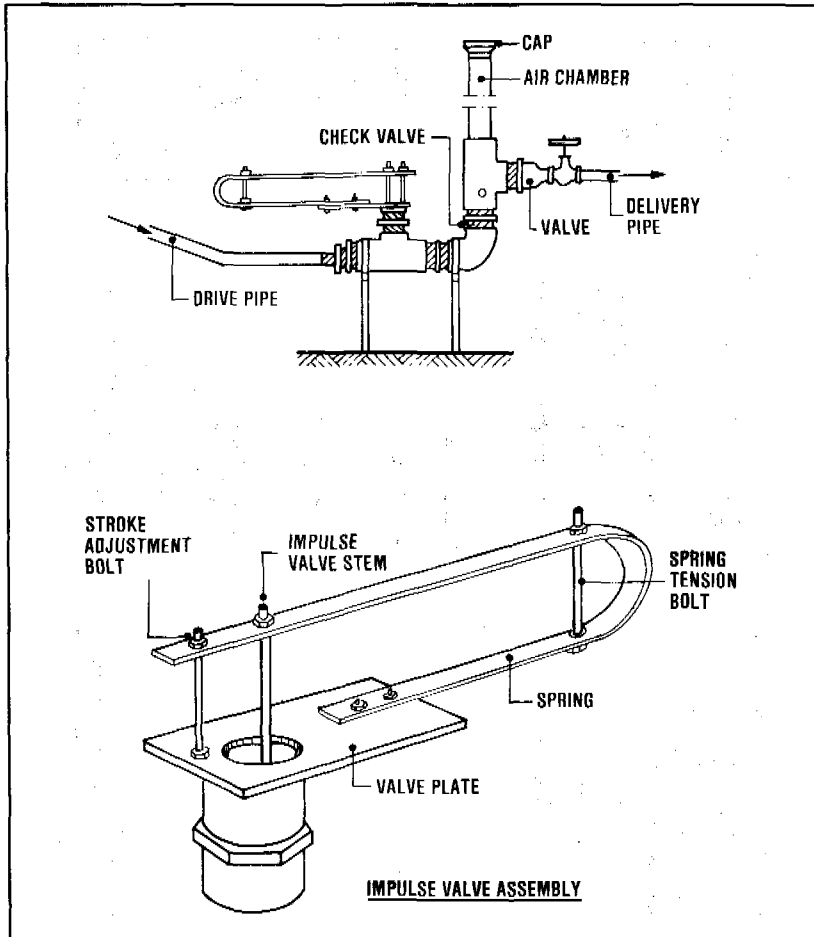
Figure 10.16. Typical hydraulic ram
