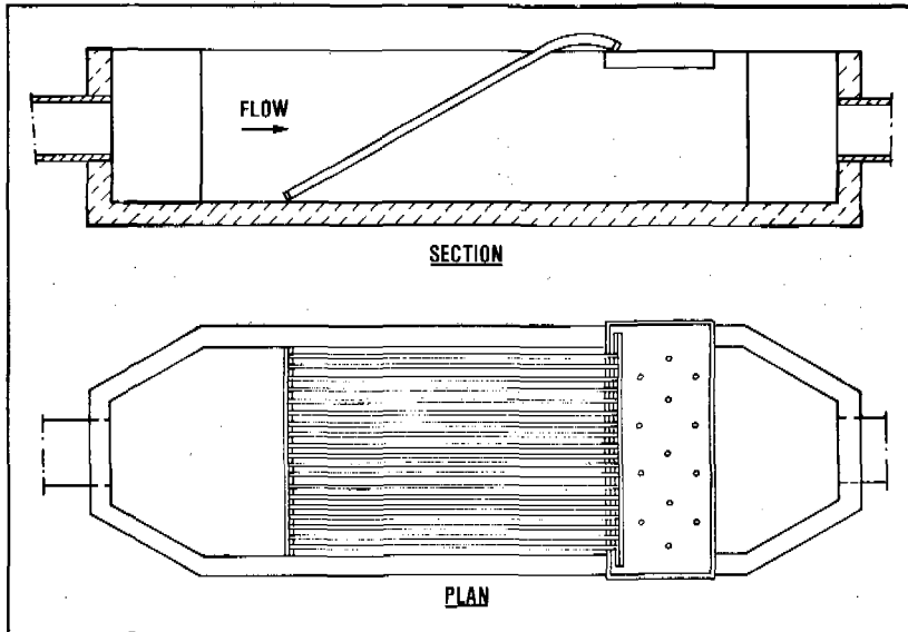
Figure 8.10. Fixed bar screen
