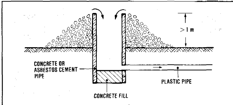
Figure 8.7. Intake structure at bottom of shallow lake.
