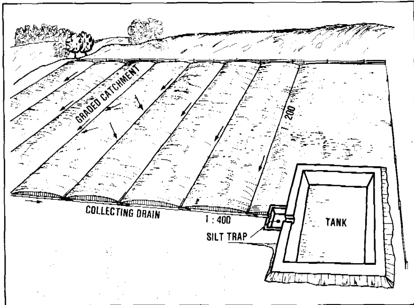
Figure 5.4. Ground catchment
