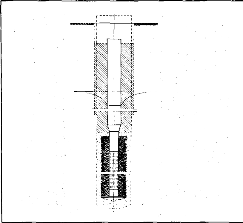
Figure 4. Well with Gravel Pack.
