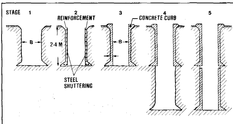
Figure 7.25. Reinforced concrete curb built on site
