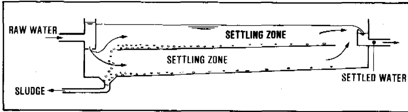
Figure 14.2. Settling tank with extra bottom
