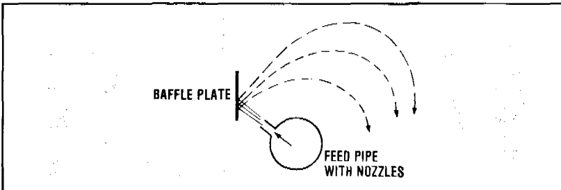
Figure 12.8. Simple spray aerator using baffle plate
