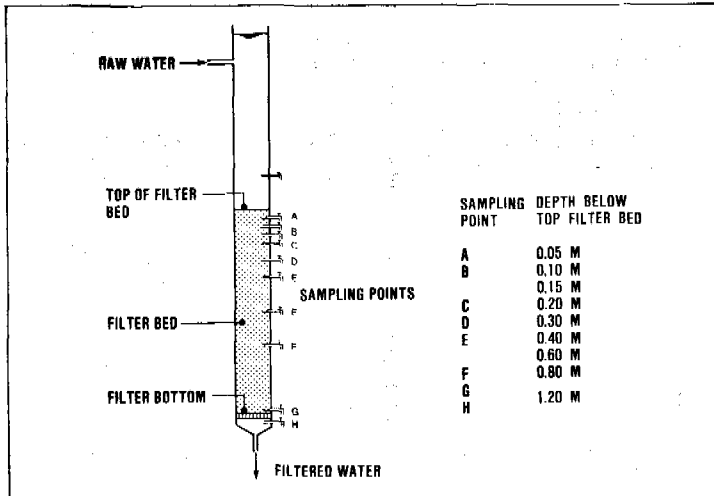
Figure 9 Experimental filter
