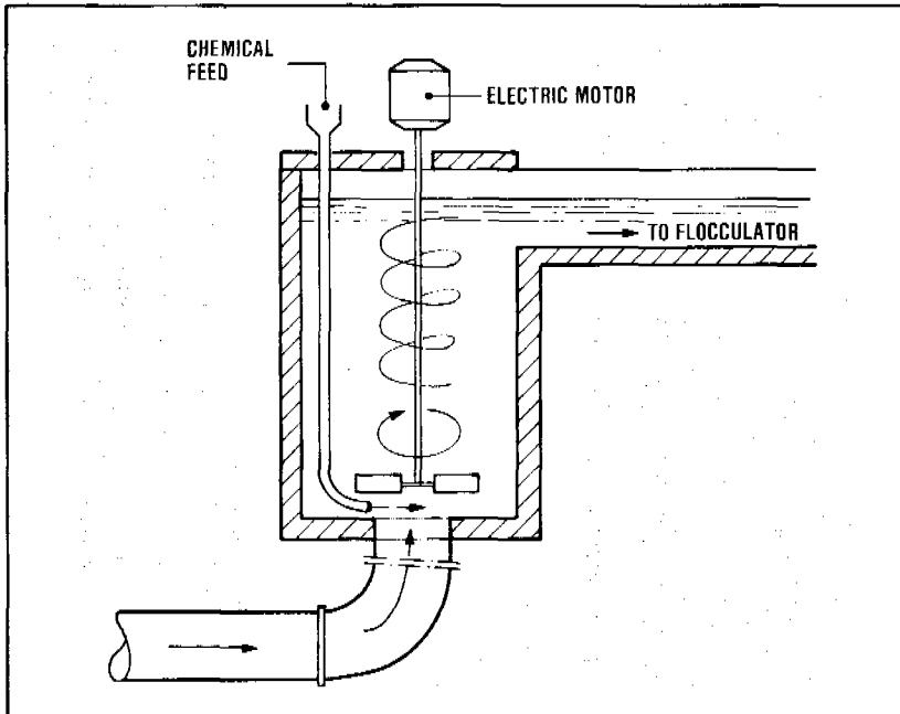
Figure 13.7. Mechanical mixer
