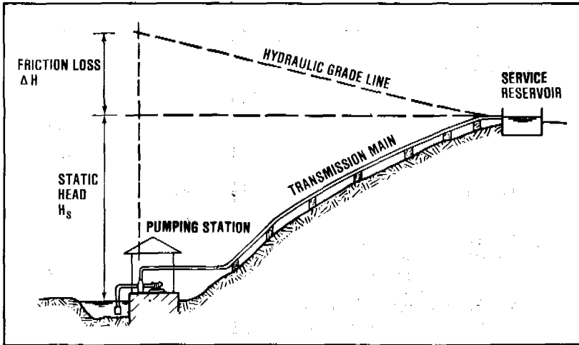
Figure 18.9. Pumped supply
