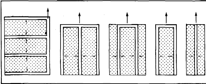
Figure 16.16. Typical arrangements of wash-water troughs
