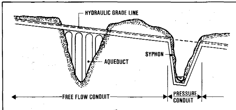
Figure 18.3. Combined free-flow/pressure conduit
