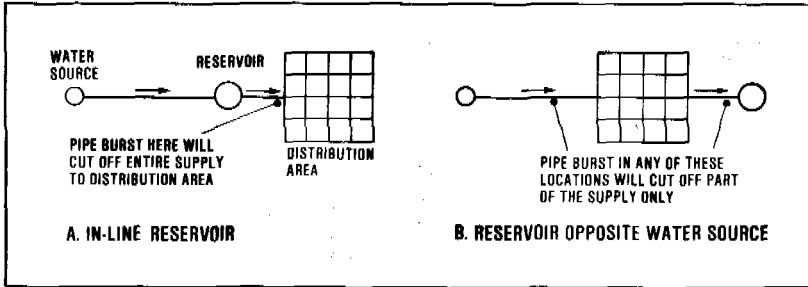
Figure 19.13. Reservoir siting
