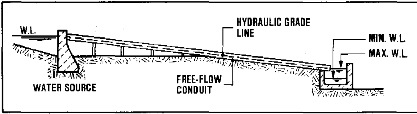
Figure 18.1. Free-flow conduit
