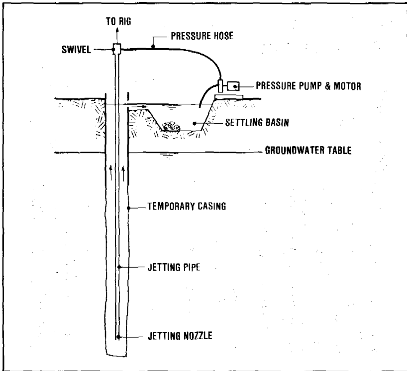
Figure 7.39. Well jetting
