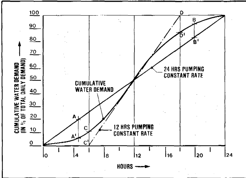
Figure 19.12. Graphical determination of required storage volume (service reservoir)
