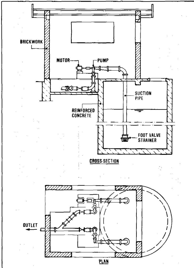
Figure 18.12. Pumping station with horizontal pumps (self-priming)
