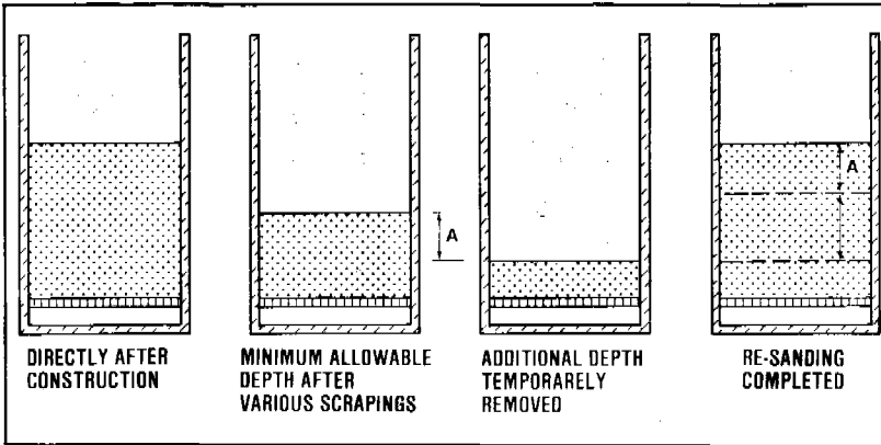
Figure 15.15. Re-sanding of a slow sand filter
