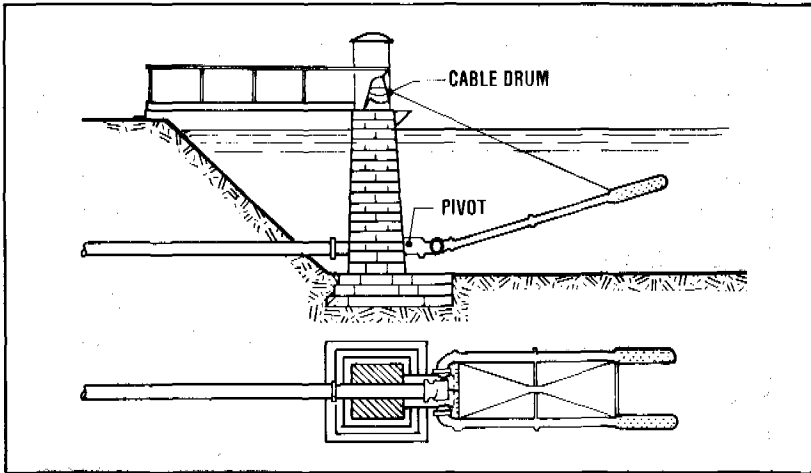
Figure 8.6. Variable depth lake water intake.
