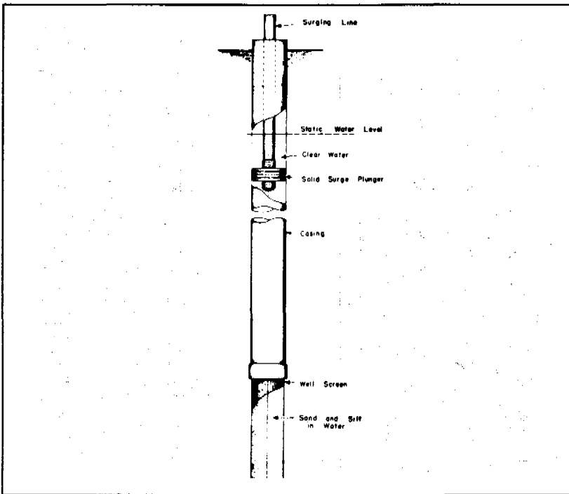
Figure 5. Surging for well development.
