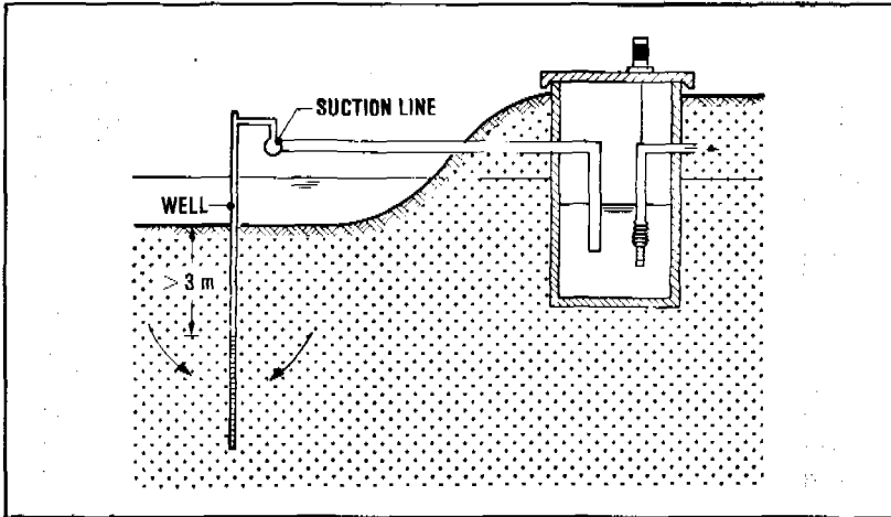
Figure 9.6. Line of wellpoints placed in riverbed
