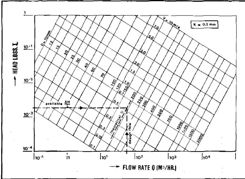
Figure 18.7. Head loss determination graph
