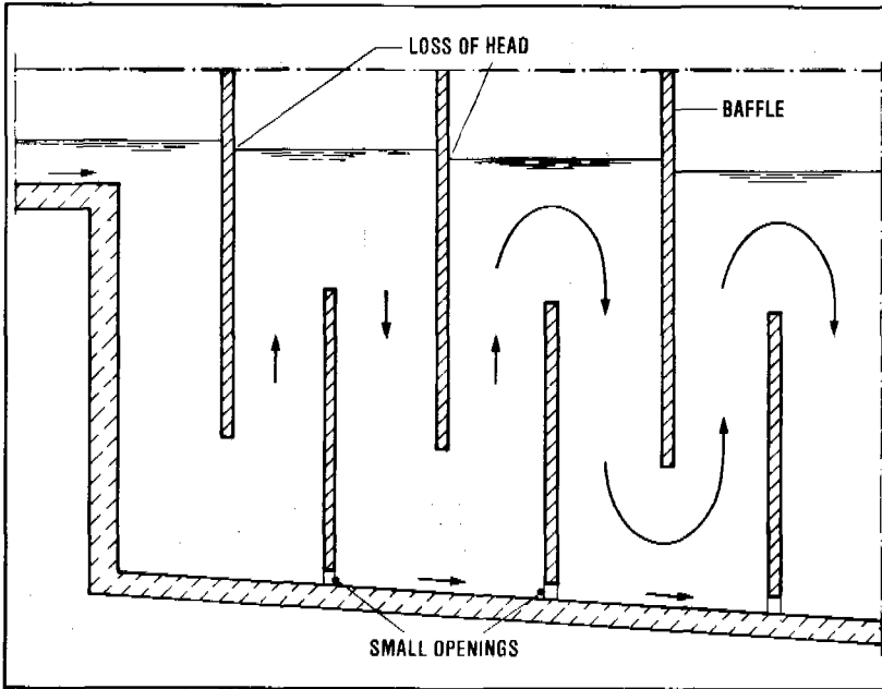
Figure 13.9. Vertical-flow baffled chamber flocculator (cross section)
