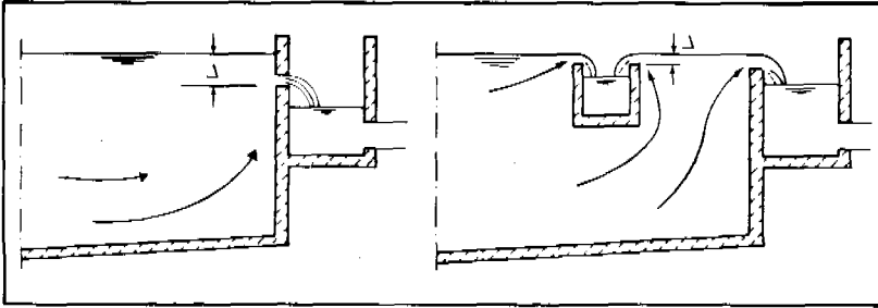
Figure 14.4. Outlet arrangements
