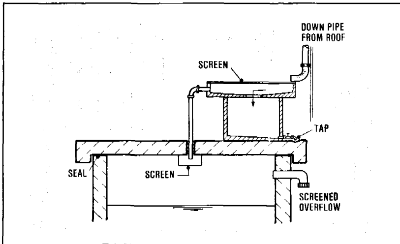
Figure 5.2. Arrangement for diverting the 'first foul flush'
