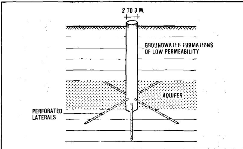
Figure 7.14. Radial collector well*
