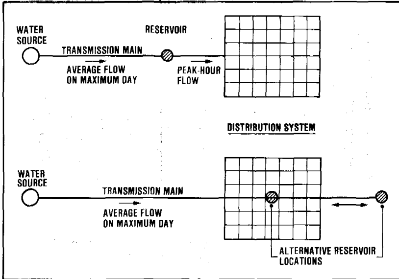
Figure 18.5. Transmission main and service reservoir (schematic)
