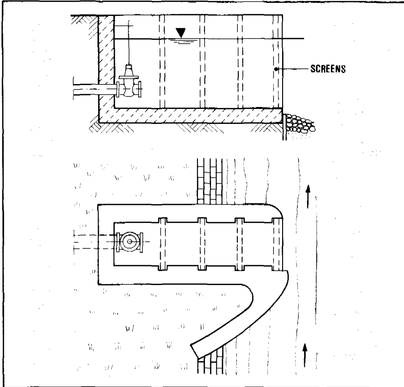
Figure 8.2. River intake structure
