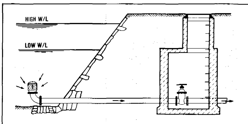
Figure 8.1. Unprotected river intake
