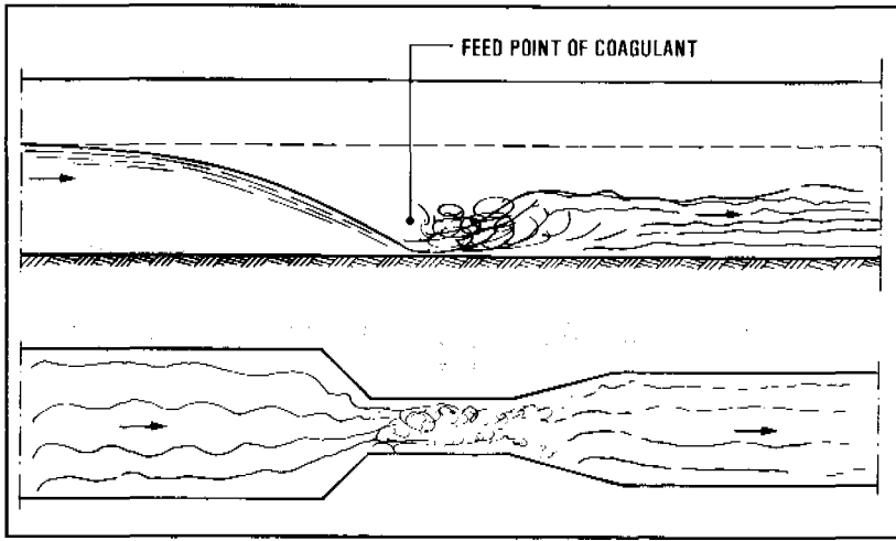
Figure 13.5. Hydraulic jump
