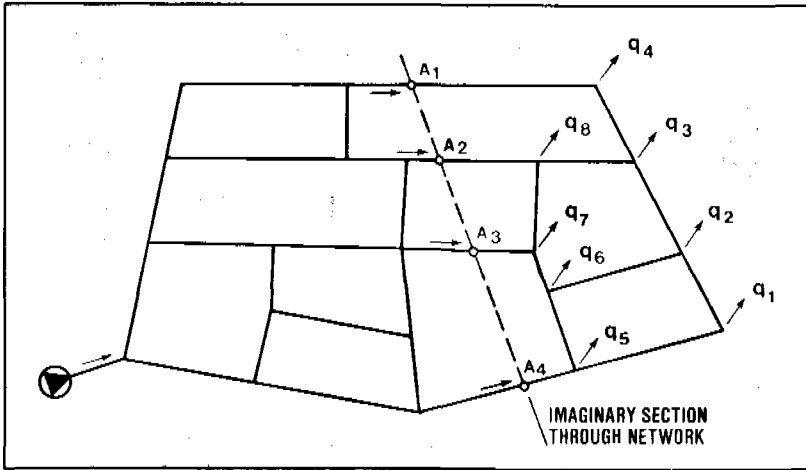
Figure 19.19. Imaginary section design method
