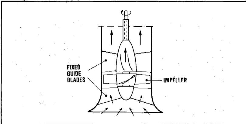
Figure 10.10. Axial-flow pump
