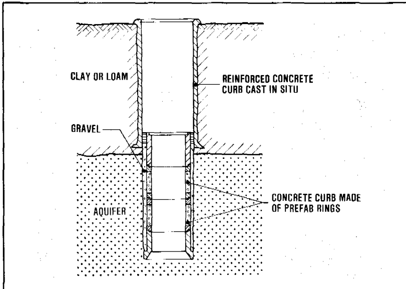
Figure 7.31. Dug well construction using combination of methods
