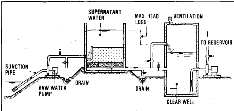
Figure 15.4. Simplified slow sand filter
