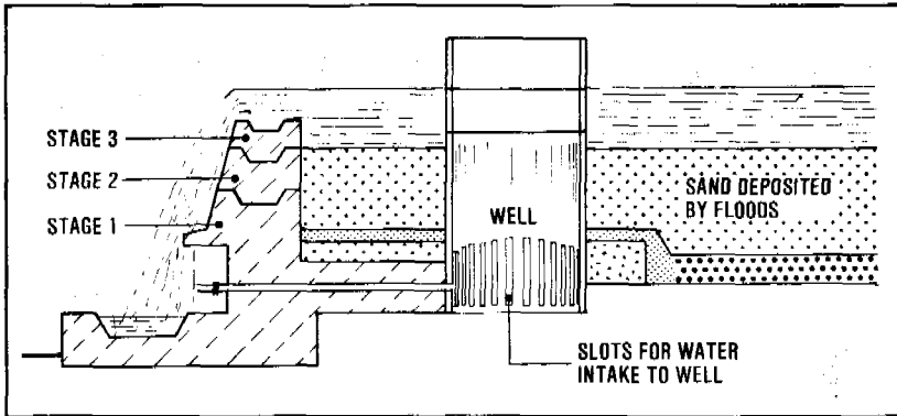
Figure 9.15. Sand dam (schematic)
