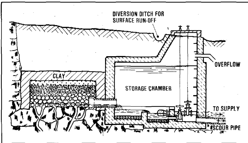
Figure 6.11. Artesian depression spring
