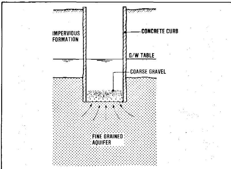
Figure 7.21. Dug well in fine granular aquifer
