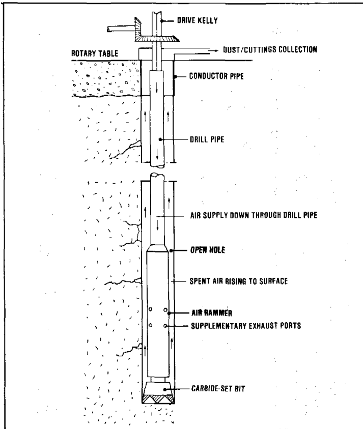
Figure 6 'Down-the-hole' hammer drill
