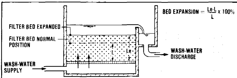
Figure 16.12. Backwashing of rapid filter
