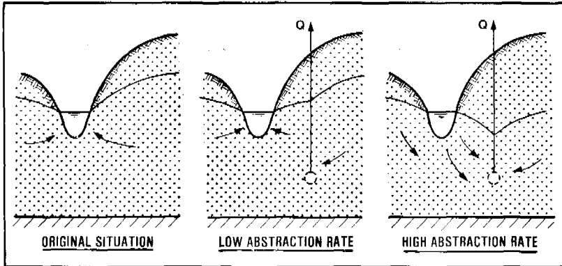
Figure 9.3. Bank infiltration
