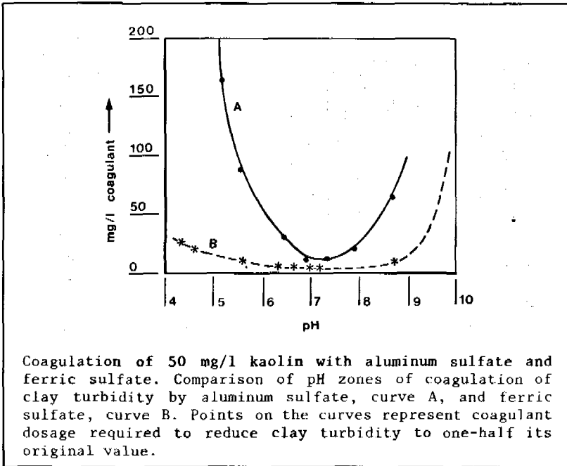
Figure 13.1. pH zone-coagulation relationship
