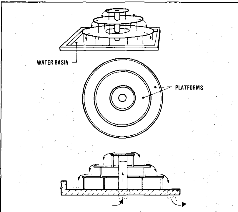
Figure 12.5. Multiple-platform aerator
