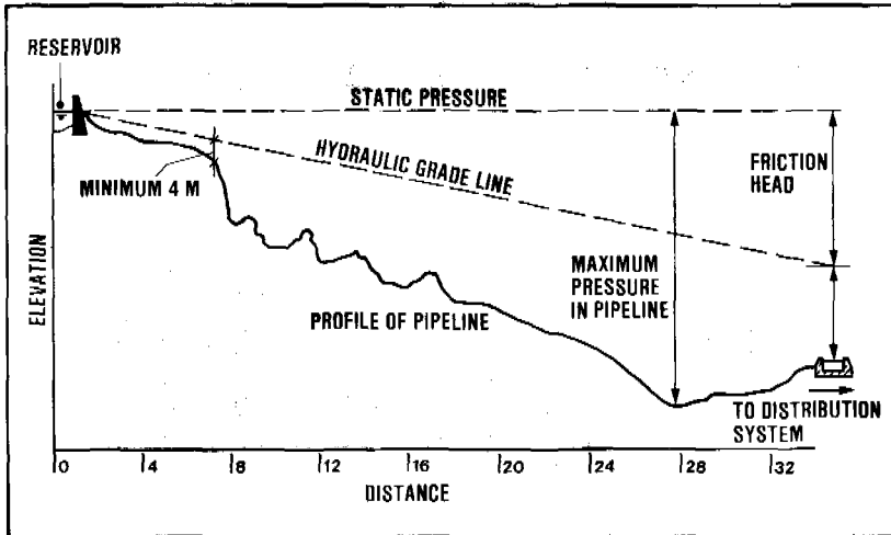
Figure 18.6. Design pressure determination for pipeline
