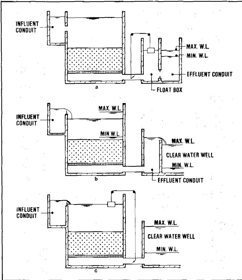
Figure 16.10. Filter control systems
