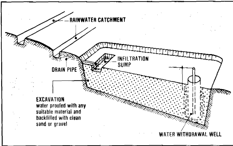
Figure 9.14. Artificial recharge using rainwater
