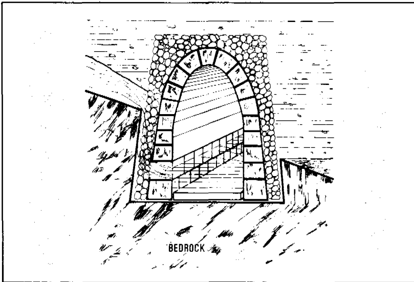
Figure 6.9. Tunnel for tapping gravity overflow spring
