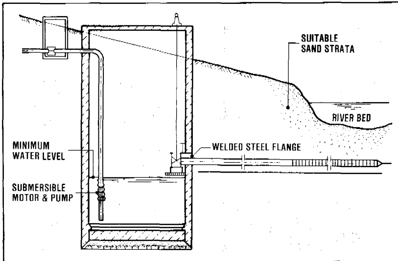
Figure 8.4. Bank river intake using infiltration drains
