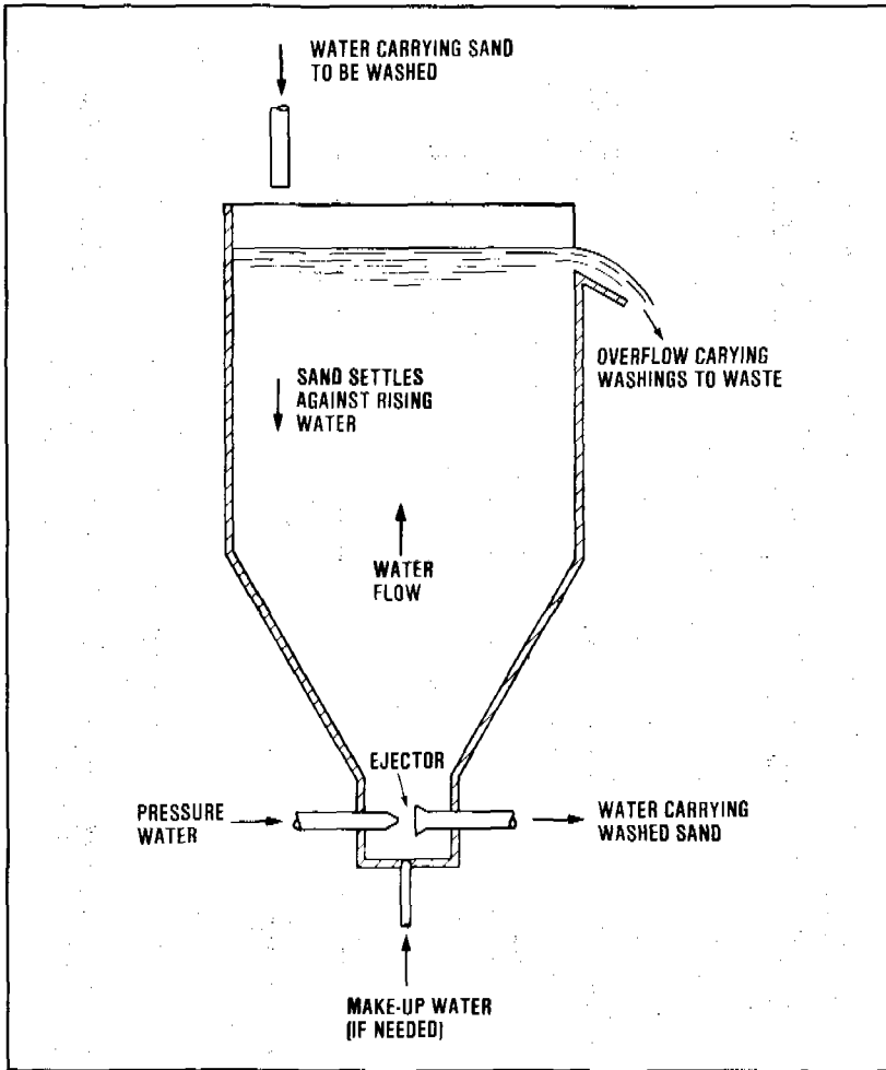
Figure 15.13. Sand washer
