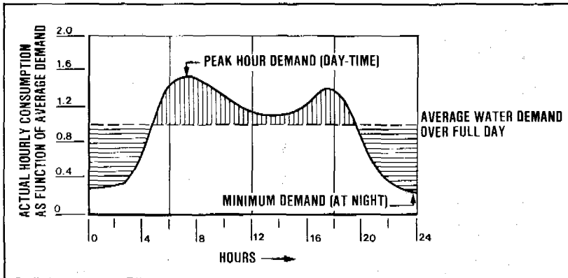
Figure 19.10. Variation of water demand during the day
