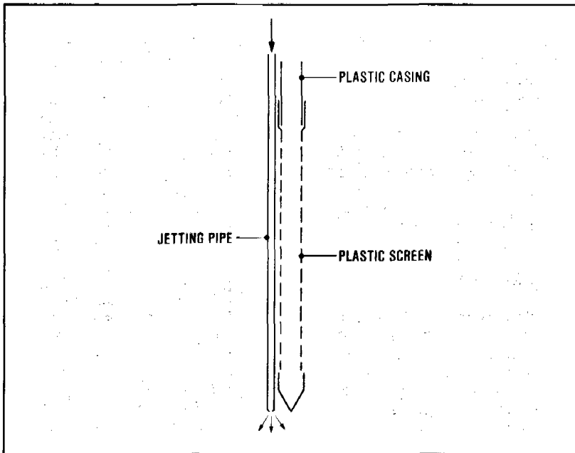
Figure 7.40. Well jetting with an outside jet pipe
