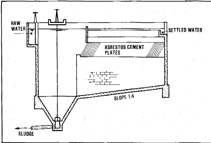
Figure 14.10. Settling tank with tilted plates
