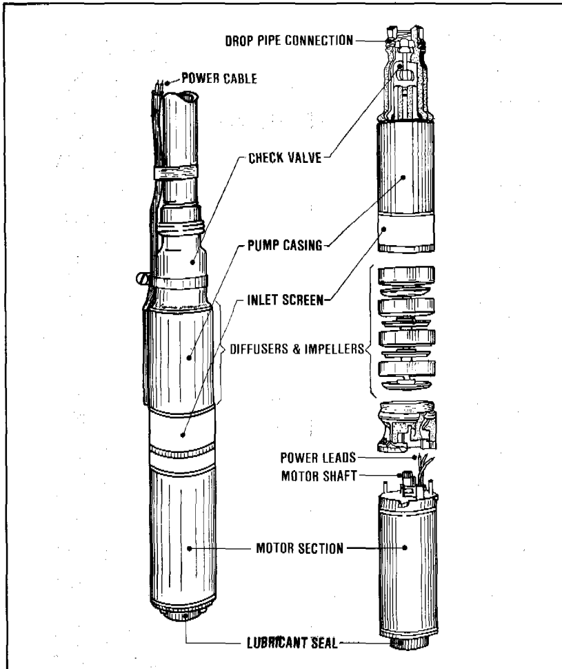
Figure 10.14. Submersible pump (exploded view)
