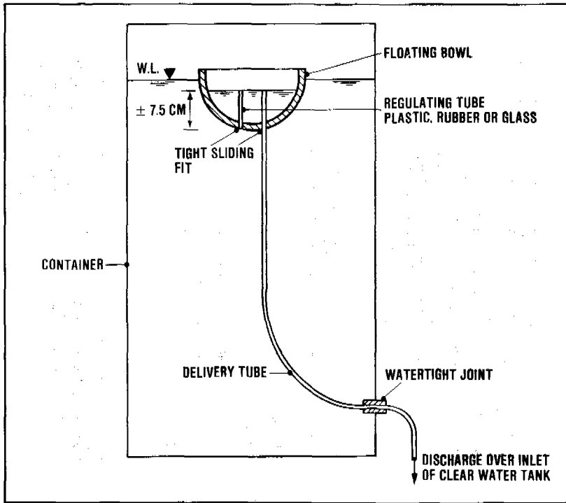
Figure 17.5. Constant-head solution feeder for chlorine compounds
