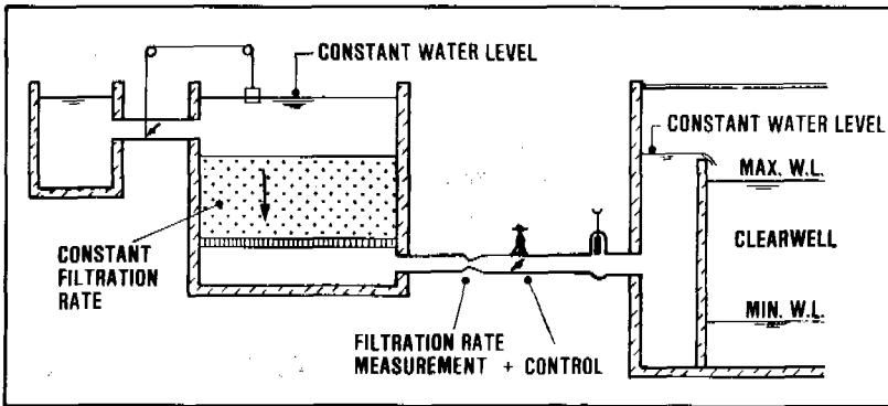
Figure 16.9. Filter-rate control
