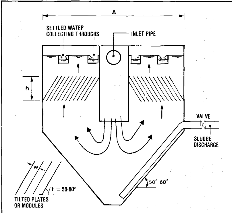
Figure 14.11. Tilted plate settling tank design parameters
