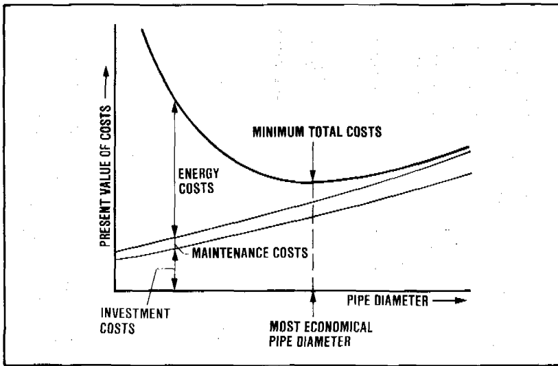
Figure 18.10. Determination of most economical pipe diameter
