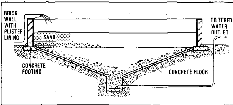
Figure 15.8. Simple slow sand filter
