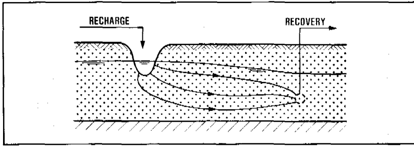
Figure 9.1. Artificial recharge of aquifer
