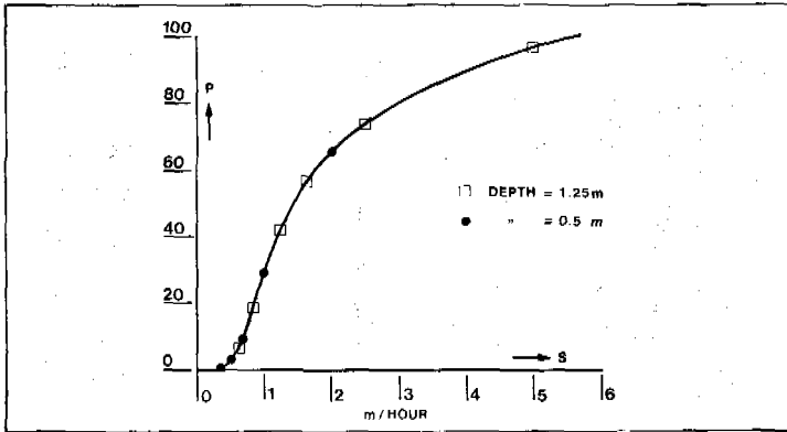
Figure 4 Cumulative frequency distribution of settling velocities
