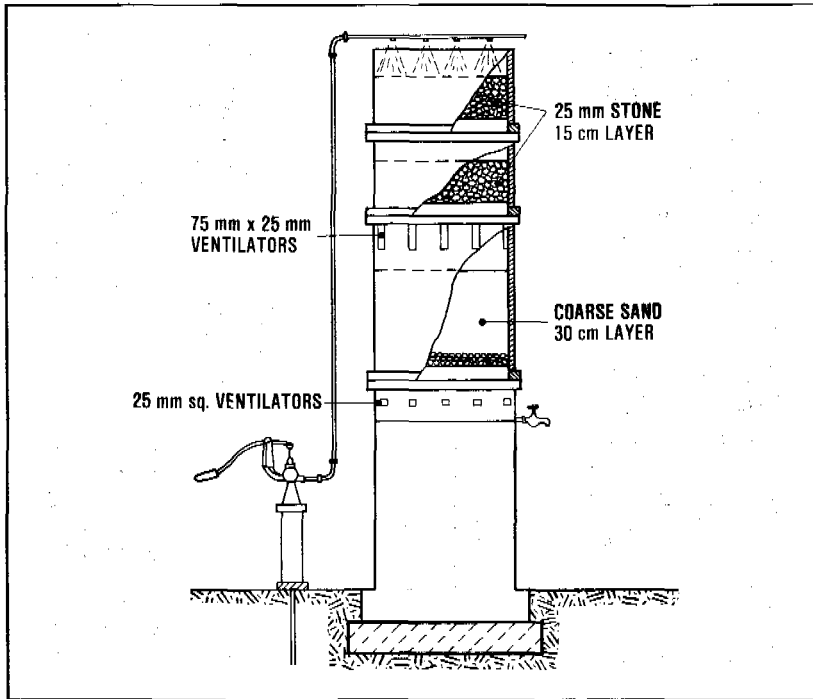
Figure 12.3. Hand-operated aeration/filtration unit
