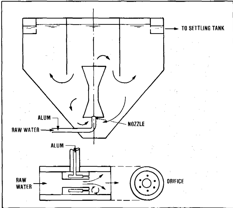
Figure 13.11. Hydraulic jet flocculator
