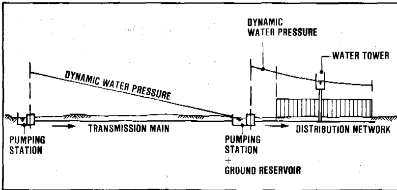
Figure 19.14. Ground reservoir with pumping station
