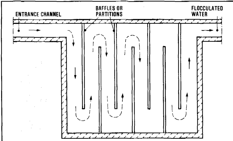
Figure 13.8. Horizontal-flow baffled channel flocculator (plan)
