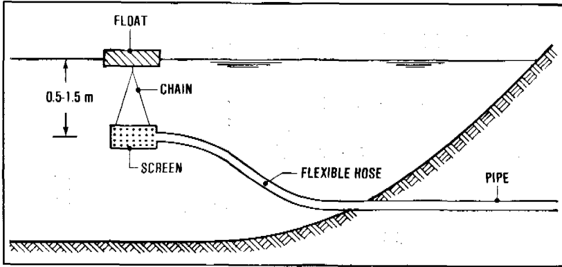
Figure 8.8. Simple water intake structure
