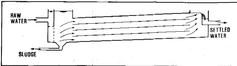
Figure 14.8. Multiple-tray settling tank
