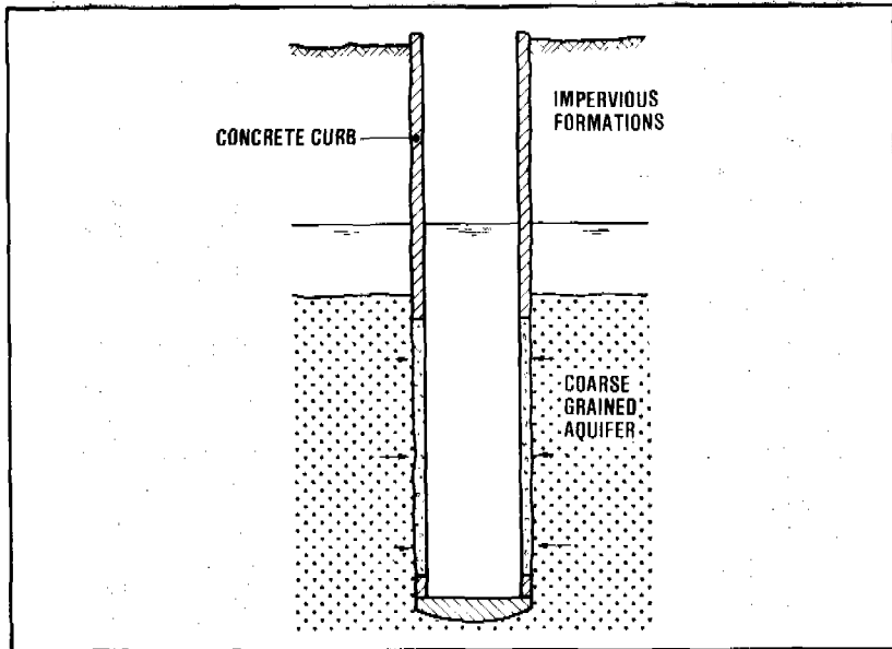
Figure 7.20. Dug well in coarse granular material
