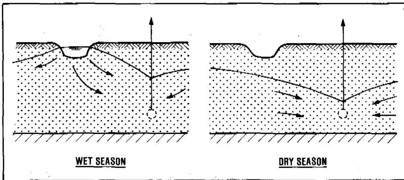
Figure 9.2. Artificial recharge with underground storage of water
