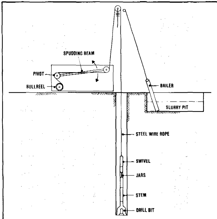
Figure 1 Cable tool or percussion drilling rig
