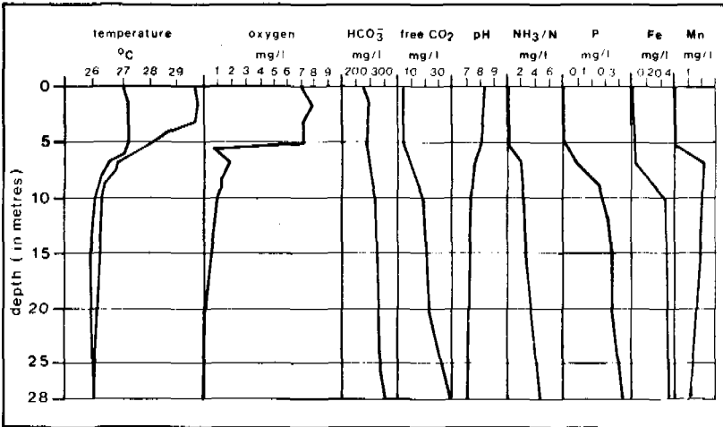
Figure 8.5. Water quality variation with depth in a deep lake (Indonesia)
