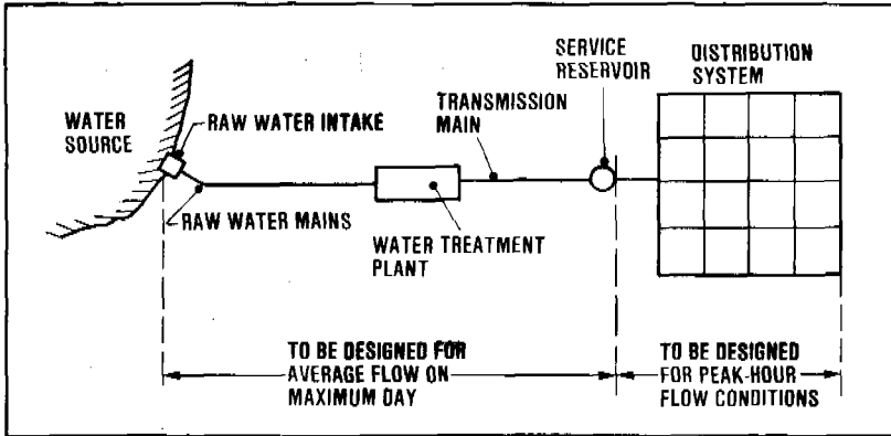
Figure 19.11. Design capacities for water supply systems components
