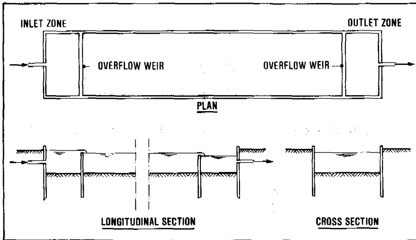
Figure 14.6. Settling basin constructed with wooden sheet piles
