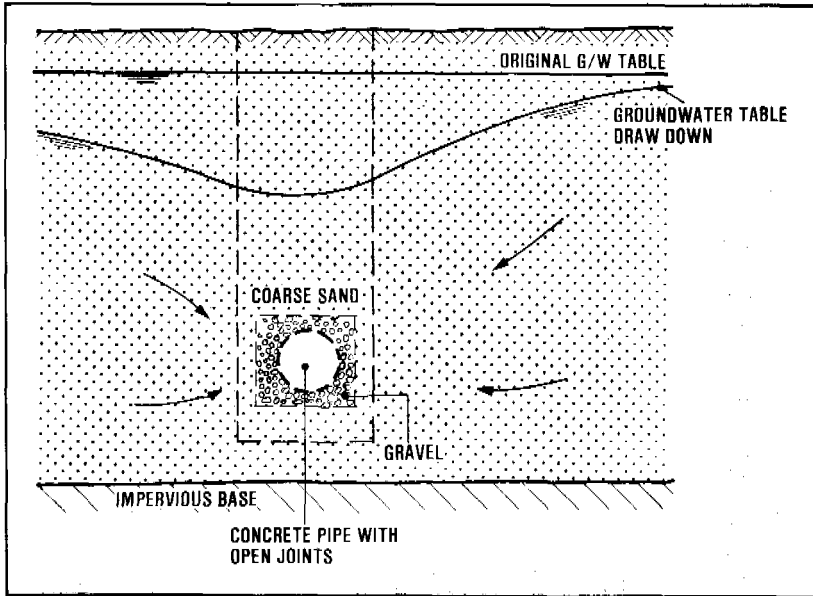
Figure 7.9. Infiltration drain
