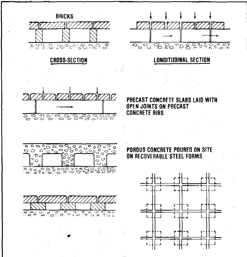
Figure 15.9. Types of filter bottoms
