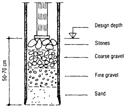
Fig 74 If the borehole is finished half-way into an aquifer, a proper filter must prevent the sand from entering before the PVC pipe is installed
