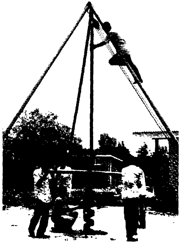
Fig. 67. The drill is kept in vertical position.
