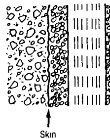
Fig 93 The "skin" between gravel pack and aquifer has to be removed
