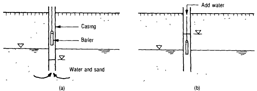
Fig 48 The casing has to be lowered while bailing and is rotated clockwise
