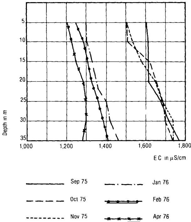
Fig. 16 Recorded E.C. values in a borehole in Mbuo Valley, Mtwara Source: Reference [12]
