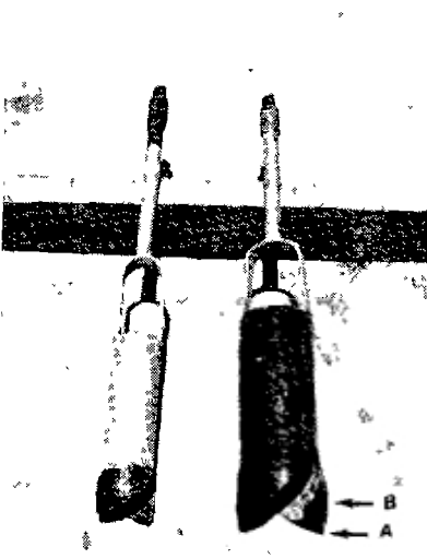
Fig. 139 Riverside augers.
