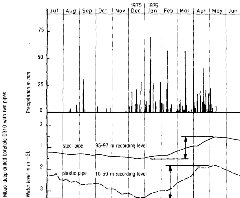
Fig 14 Recorded groundwater levels in a borehole in Mbuo Valley, Mtwara Source Reference [12]
