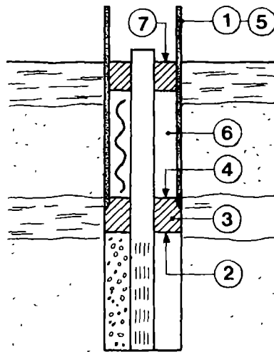
Fig 103 The procedure for installing clay seals and backfill. The circled numbers correspond to the text.
