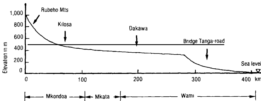
Fig 31 The longitudinal profile of the Wami River.
