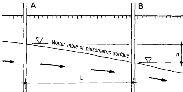
Fig. 10. The gradient of the groundwater table between A and B is defined as i = \frac{h}{L}
