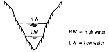
Fig 22. In the upper course of a river no suitable sediments are found.
