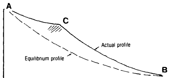
Fig. 27. A discontinuity in the longitudinal profile of a river caused by more resistant rocks at point C.
