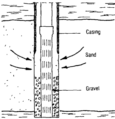
Fig. 88 The casing is pulled up too far during installation of the gravel pack. sand from the aquifer fills the gap!
