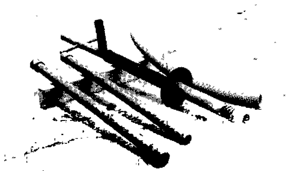
Fig. 153. Disassembled survey test pump. rising mains (one with ball valve), superstructure and hose. Note the two springs in the pump.
