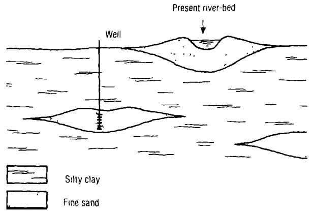
Fig. 39 Buried riverbeds offer good prospects for wells
