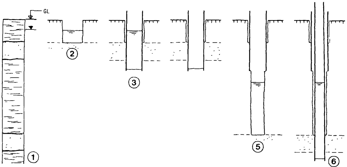
Fig 76 The successive stages of telescopic drilling. The circled numbers correspond to the text
