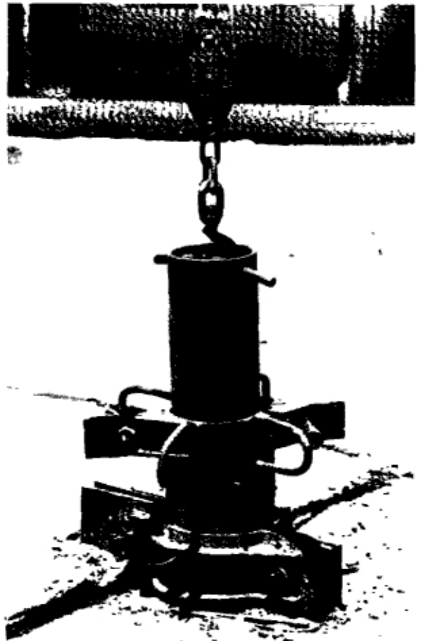
Fig. 75. With telescopic drilling a smaller size casing is inserted into the outer one, which seals off the upper aquifer.
