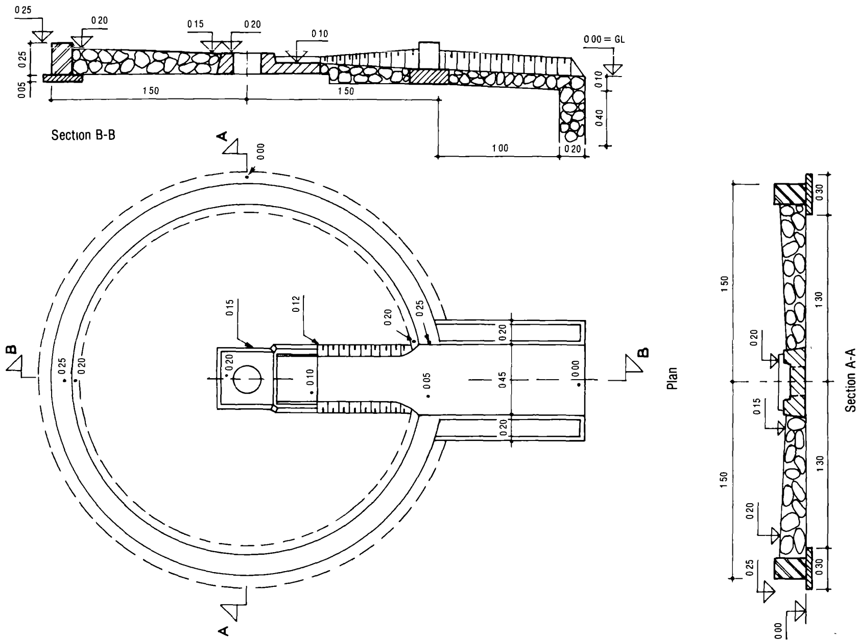
Fig 105. Design of the slab. Measures are given in metres.
