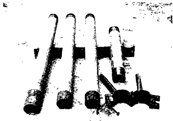
Fig 150. ABS casing pipes with steel connectors. slotted with shoe, slotted, plain, plain 0.5 m, protectoring. In the foreground a casing clamp
