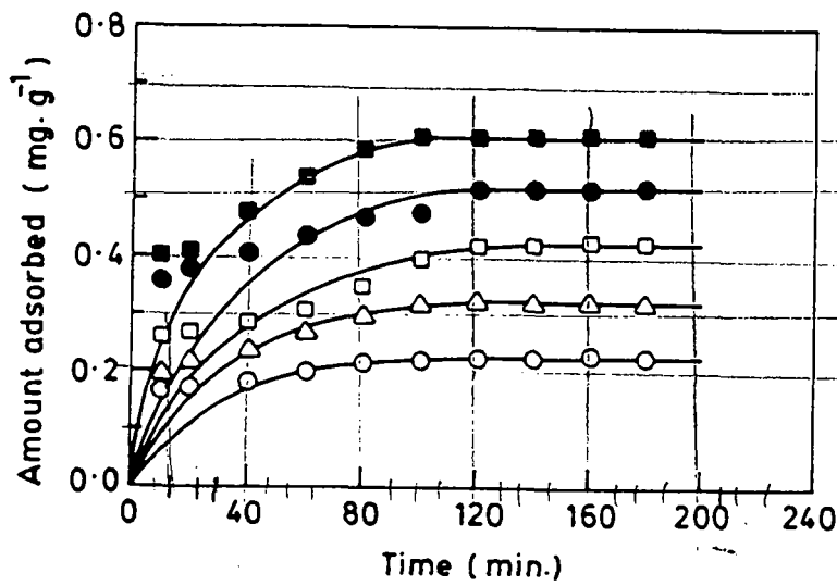
Fig. 1. Effect of concentration on removal of fluoride by fly ash, (o) 5 mg L -1 , (Δ) 7.5 mg L -1 , (□) 10 mg L -1 , (●) 12.5 mg L -1 , (■) 15 mg L -1 . Conditions: 30 °C Temperature, 6.5 pH.
