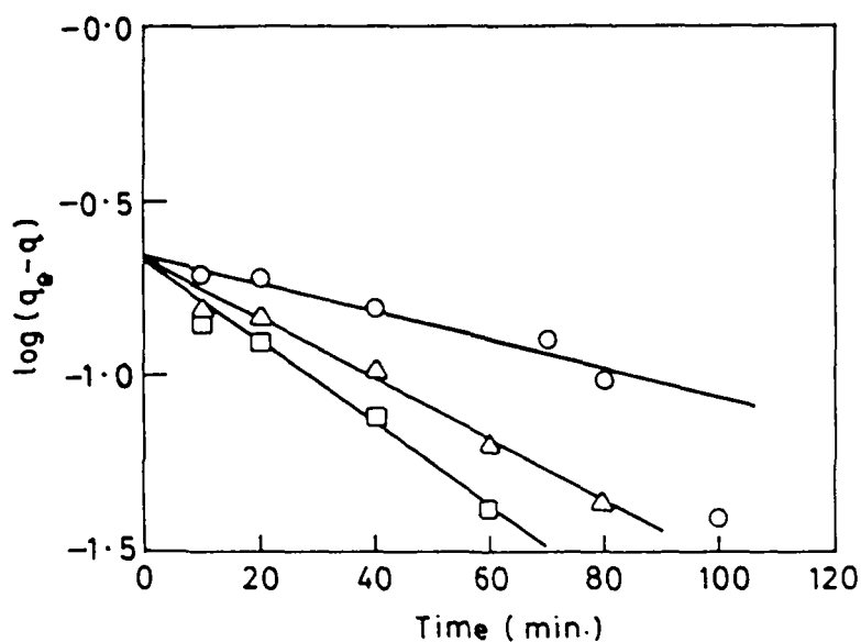
Fig. 3. Plots for rate constants of adsorption at different temperatures. (○) 30 °C, (Δ) 40 °C, (□) 50 °C. Conditions: 10 mg L -1 concentration, 6.5 pH.
