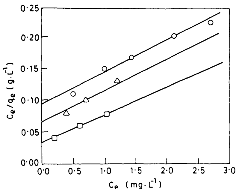
Fig. 6. Langmuir plot for the removal of fluoride by fly ash (○) 30 °C, (Δ) 40 °C, (□) 50 °C. Conditions: 6.5 pH.
