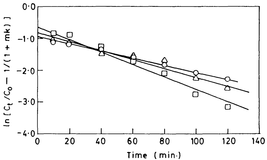
Fig. 5. Mass transfer plot (McKay et al. , 1981) for the adsorption of fluoride on fly ash, (o) 30 °C, ( \Delta ) 40 °C, ( \square ) 50 °C. Conditions: 10 mg L -1 concentration, 6.5 pH.
