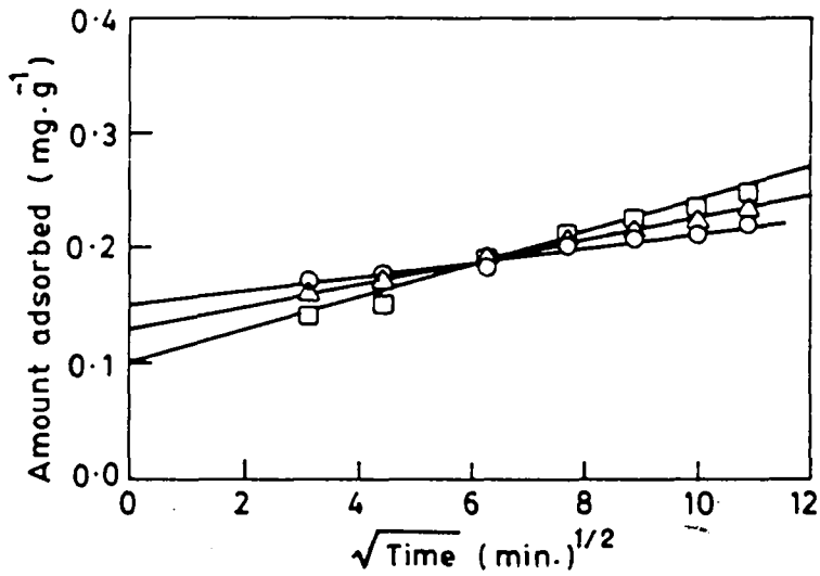
Fig. 4. Intraparticle diffusion plot for the adsorption of fluoride on fly ash, (o) 30 °C, ( \Delta ) 40 °C, ( \square ) 50 °C. Conditions: 10 mg L -1 concentration, 6.5 pH.
