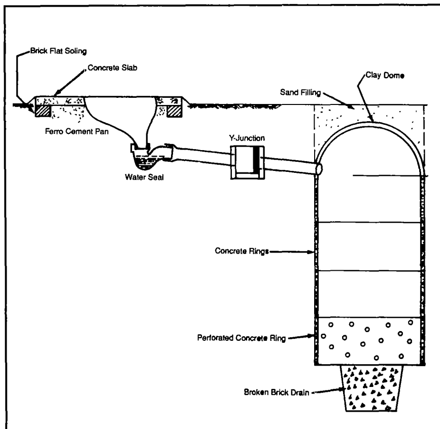
Figure 3.3. Latrine design - Section A - A
