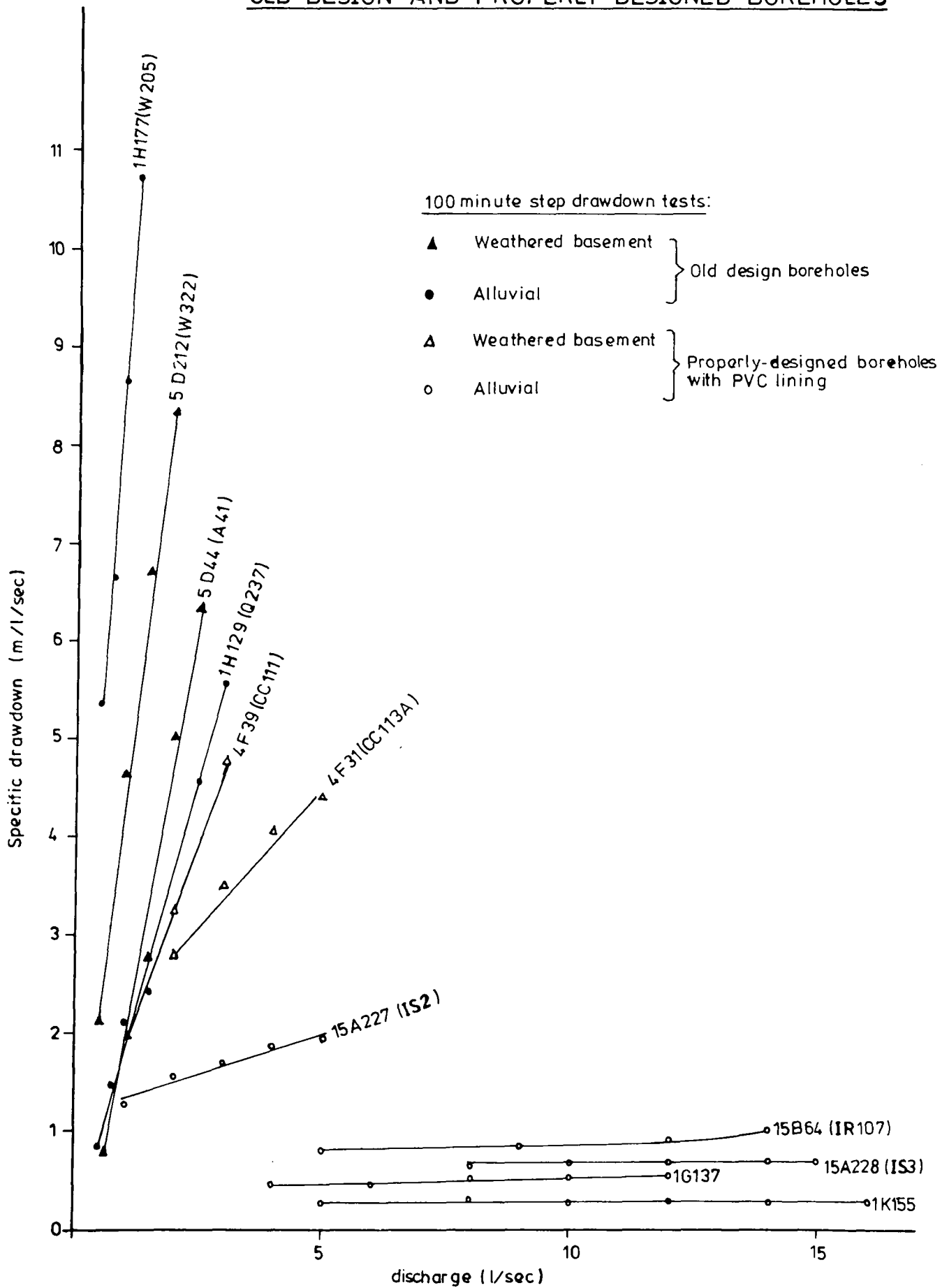
FIGURE 3.2 COMPARISON OF BOREHOLE PERFORMANCE FOR OLD DESIGN AND PROPERLY-DESIGNED BOREHOLES
