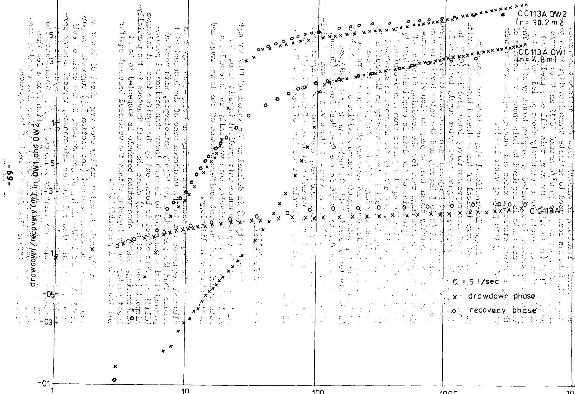
FIGURE 3.8 TEST PUMPING AT LILONGWE INTERNATIONAL AIRPORT CC 113A (4F 31)
