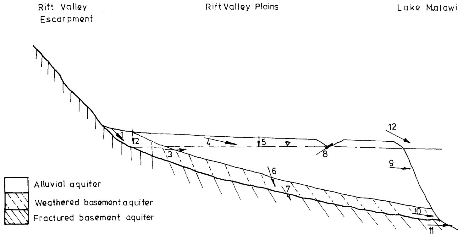
FIGURE 3.18 SCHEMATIC DIAGRAM TO SHOW RECHARGE AND DISCHARGE IN ALLUVIAL AQUIFERS
