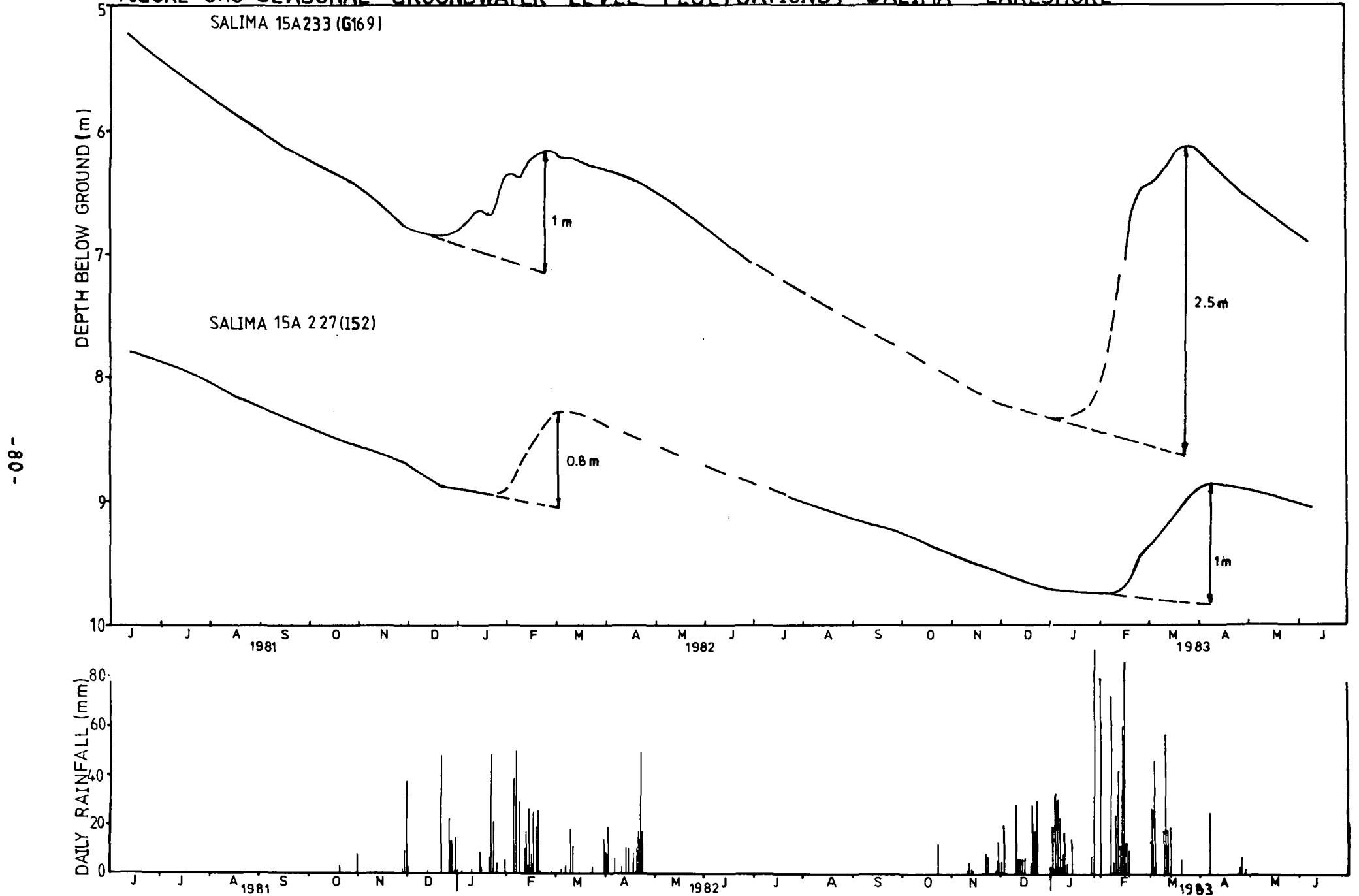
FIGURE 3.13 SEASONAL GROUNDWATER LEVEL FLUCTUATIONS, SALIMA LAKESHORE
