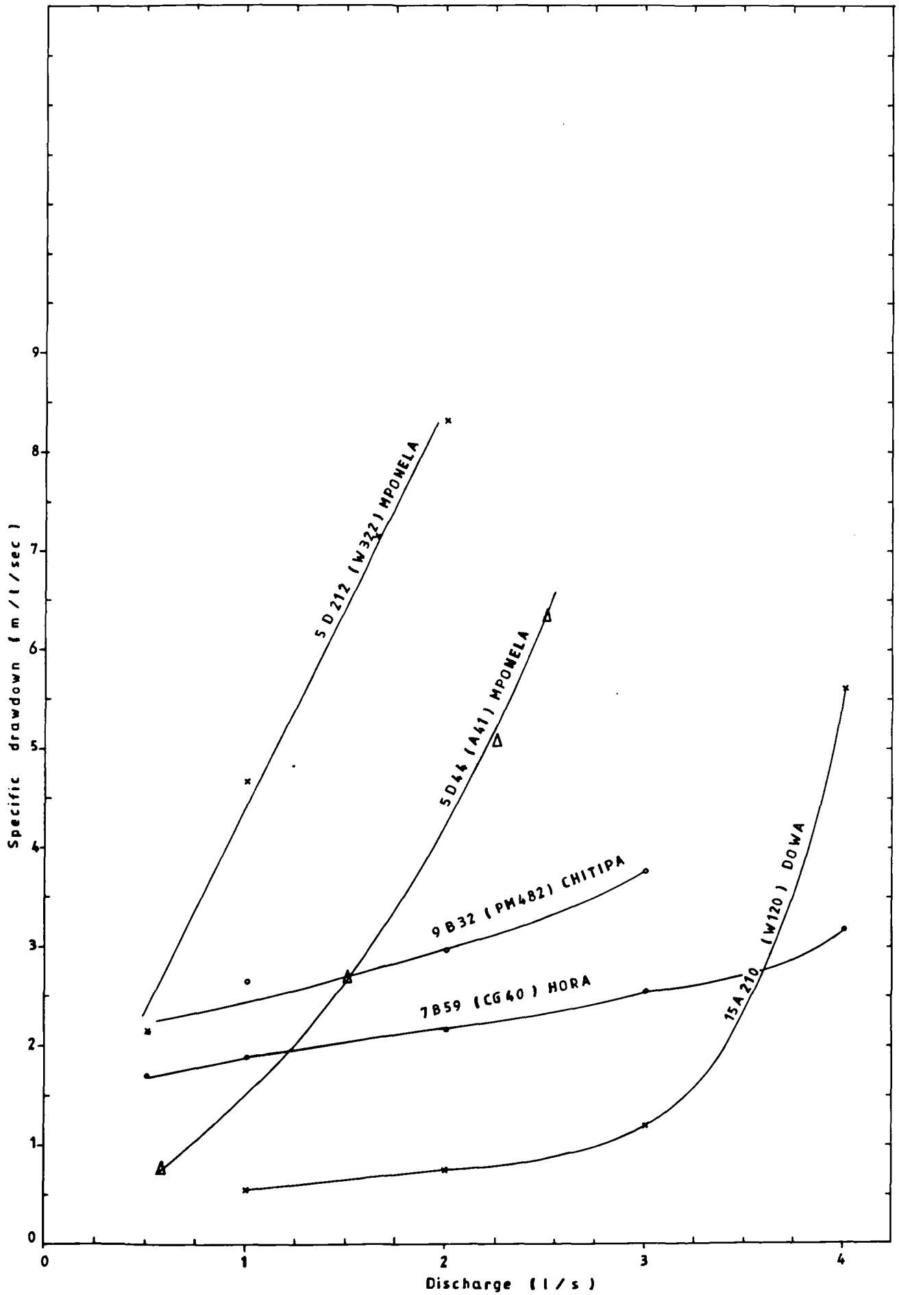
FIGURE 33 100 MINUTE STEP DRAWDOWN TESTS, BASEMENT BOREHOLES (old design)
