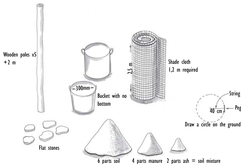
Materials required for building a "tower garden".
