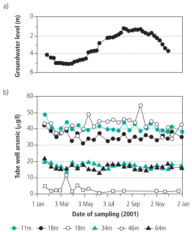
Fig. 4. a) Variations in groundwater level in the Araidhazar study area over the course of one year, based on measurements inside a monitoring well screened at 6 m below the surface. b) Time series of groundwater arsenic levels for the six private tube wells shown in Fig.1 that met the Bangladesh drinking-water standard of 50 µg/l (well depths below the ground surface are also shown)
