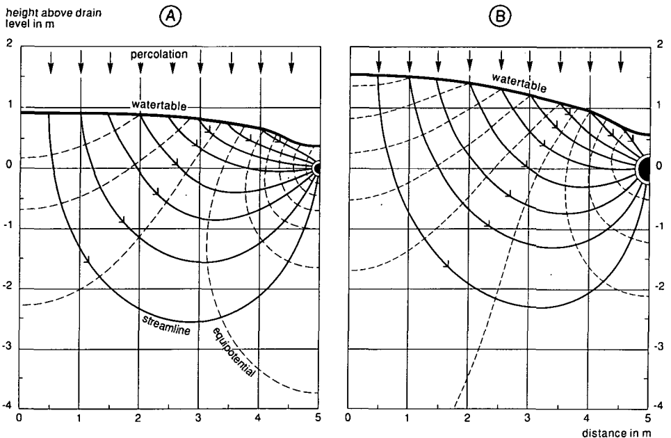
Figure 12.10 Equipotentials and streamlines of groundwater flow to drains in deep homogeneous soils A: small diameter drain, large K ; B: large diameter drain, small K (Childs 1943)
