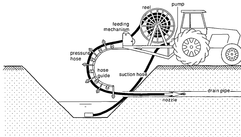
Figure 21.29 Flushing machine
