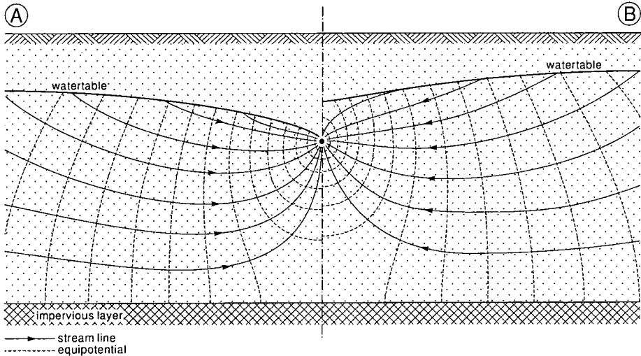
Figure 21.41 Example 21.5: Flow net showing streamlines and equipotential lines A: Ideal drain B: Non-ideal drain with a_c = 0.75
