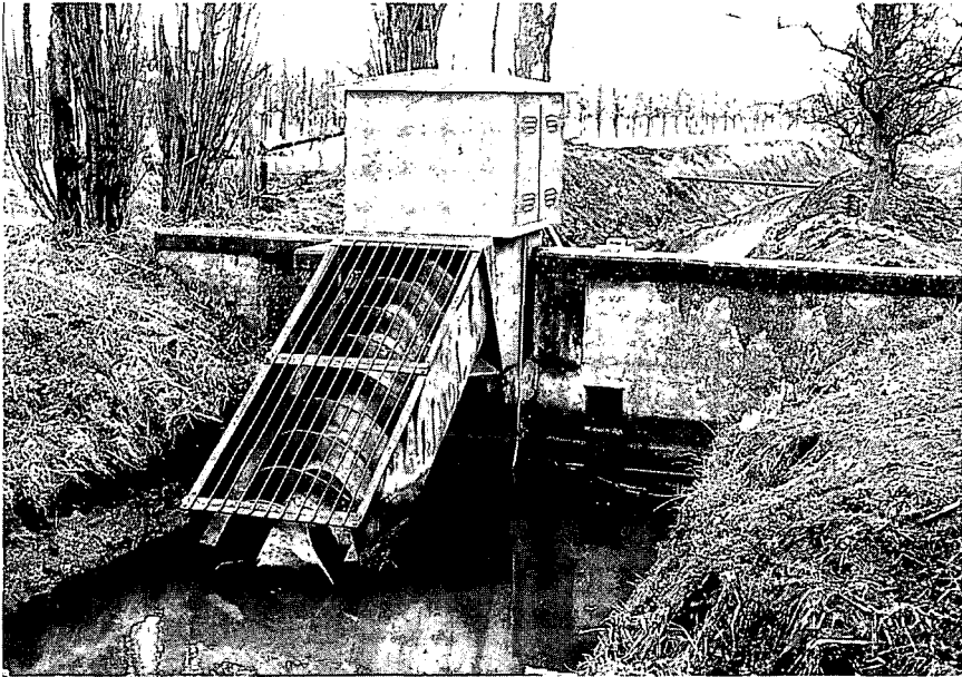
Photo 23.1 Small Archimedean screw in a drainage canal
