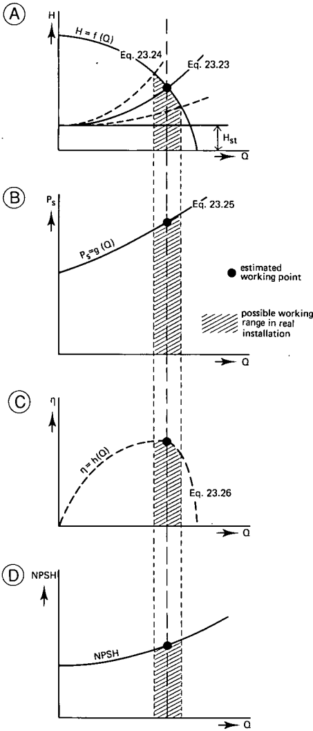
Figure 23.20 Combination of pump and pumping system
