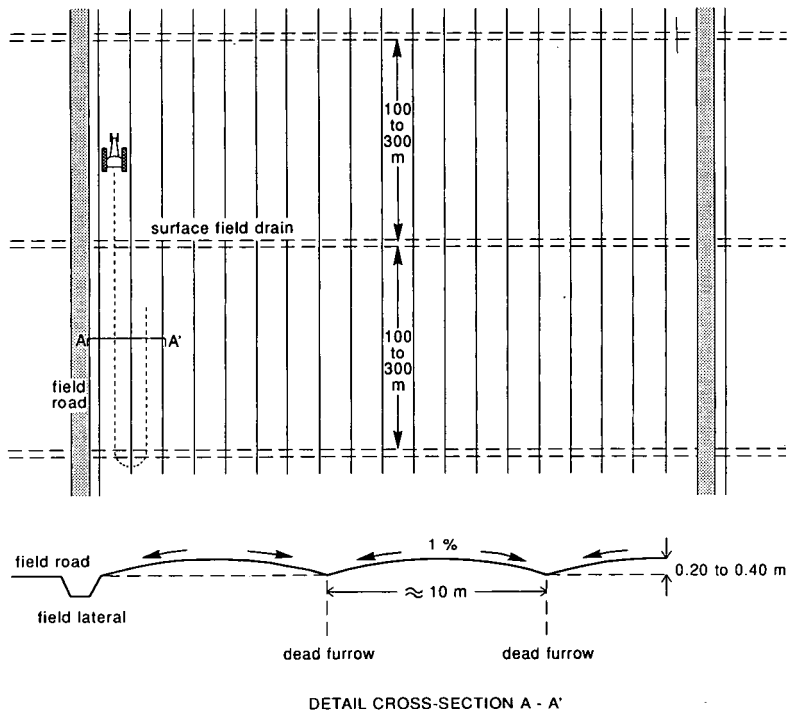
Figure 20.1 The bedding system
