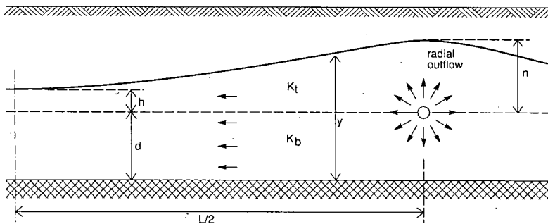
Figure 14.10 Schematic watertable for 'inverse' drainage
