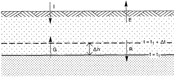
Figure 16.3 Water balance components of the unsaturated zone
