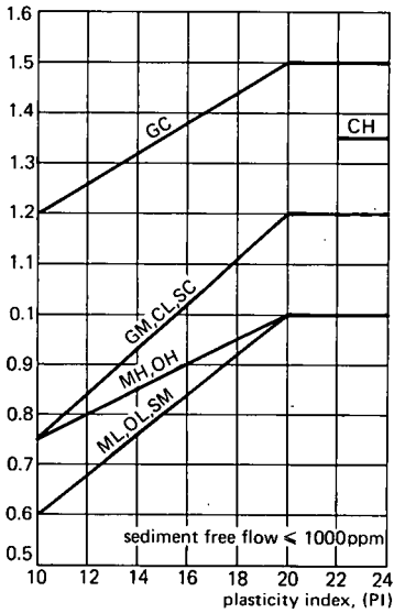
Figure 19.29 Basic allowable velocity, v_b , for coherent earthen materials, and related correction factors A through D (adapted from USDA 1977)
