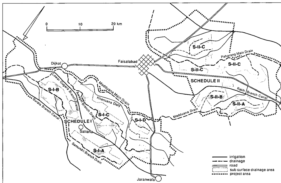
Figure 18.3 Project area and subsurface drainage area of Drainage IV Project
