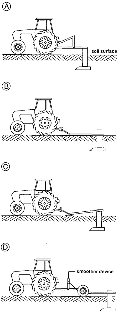
Figure 21.58 Types of mole plough
