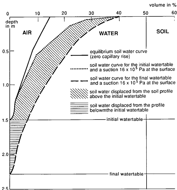
Figure 15.12 Soil water displaced by capillary rise in the case of a falling watertable (after van Hoorn 1979)
