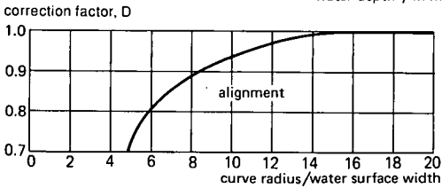
Figure 19.29 Basic allowable velocity, v_b , for coherent earthen materials, and related correction factors A through D (adapted from USDA 1977)
