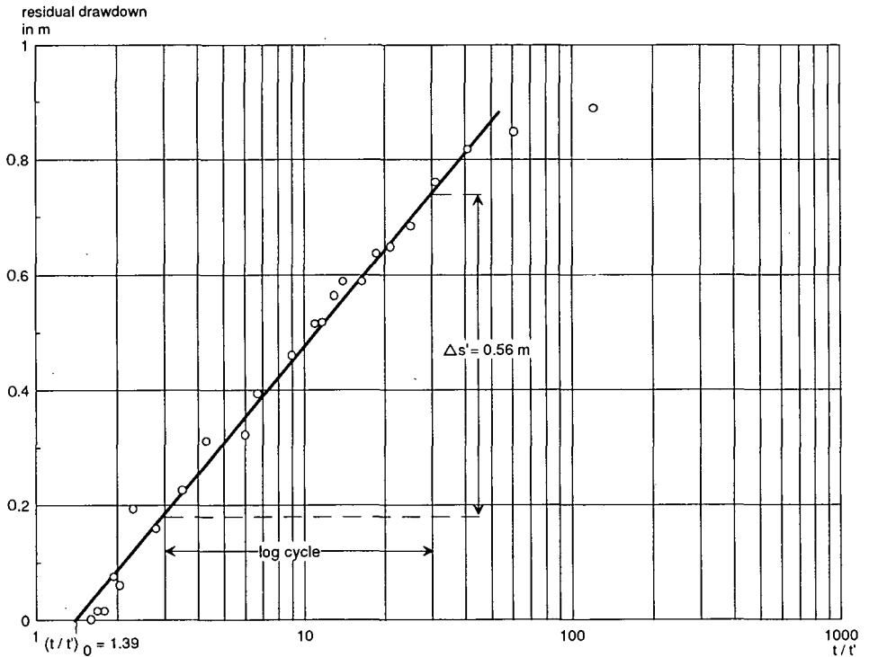
Figure 10.14 Time-residual drawdown plot of field data of a single-well test in an unconfined aquifer
