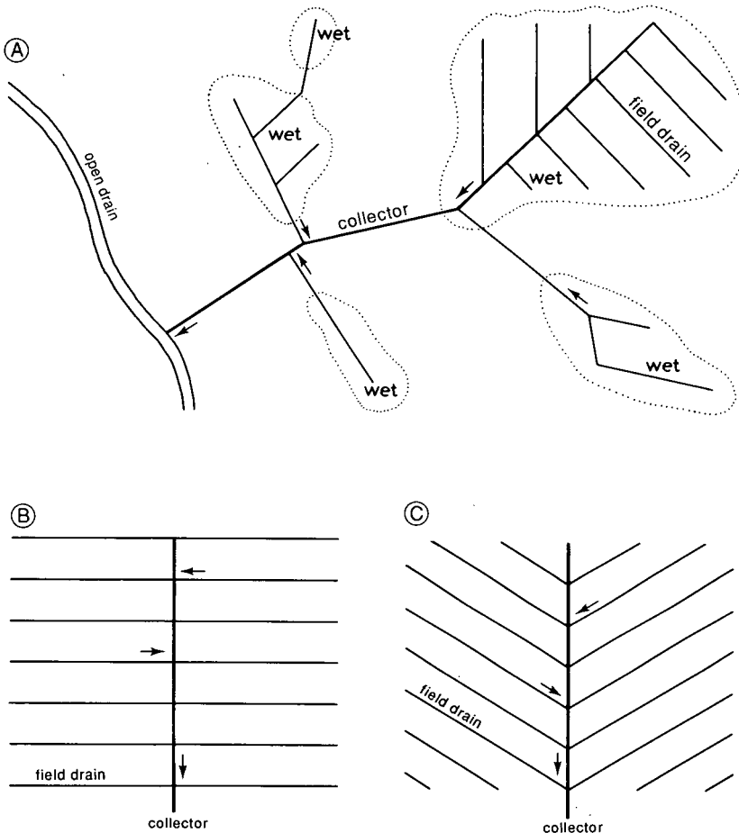
Figure 21.11 Different layout patterns for a composite pipe drainage system
