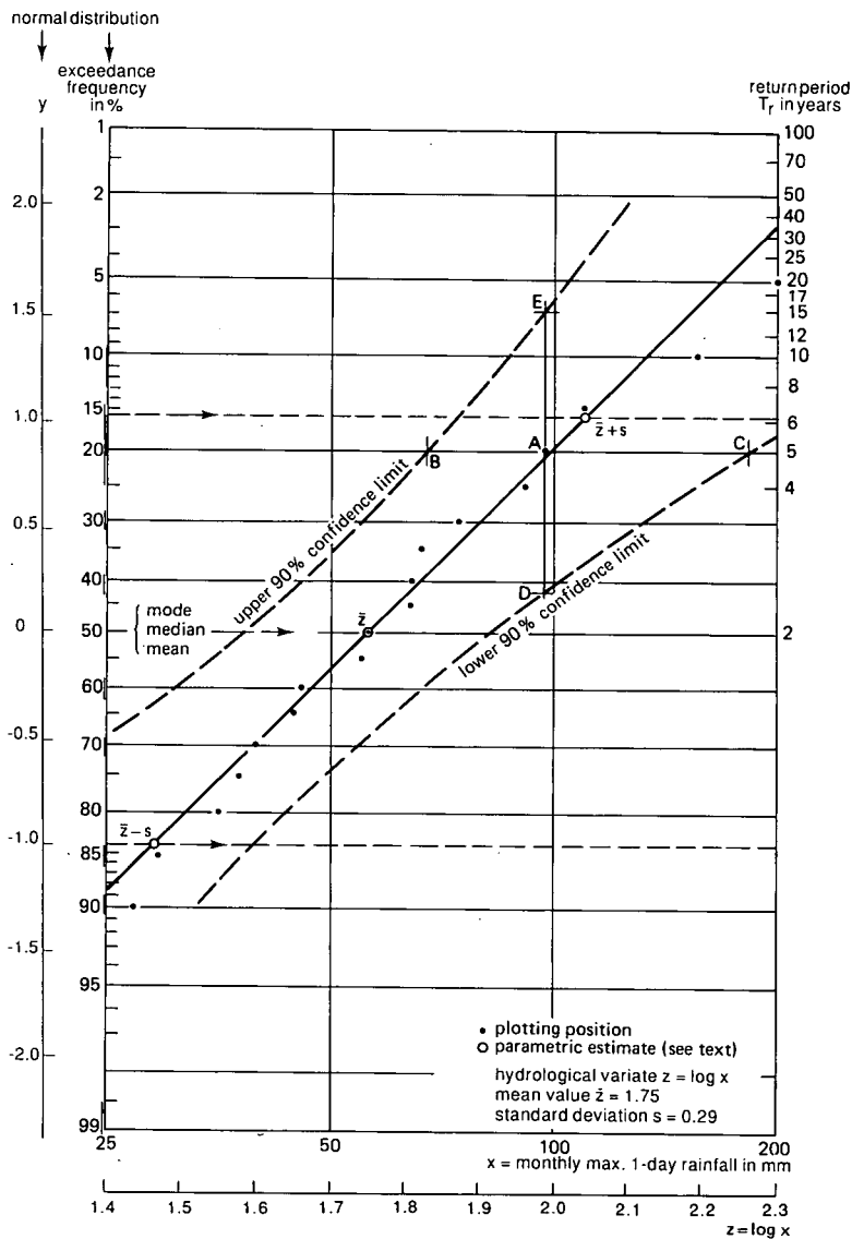
Figure 6.13 The log values of the data of Table 6.5, plotted on normal probability paper with a fitted line, based on the parametric method
