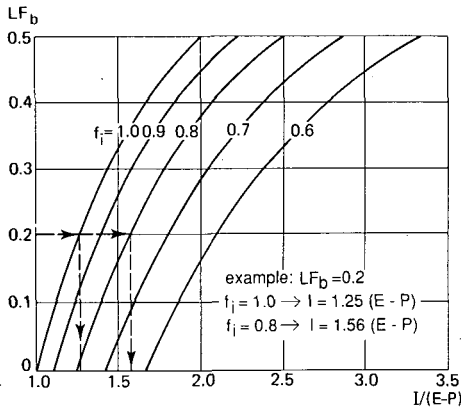
Figure 15.24 Relation between LF_b , f_i , I/(E-P) , and R^x/I
