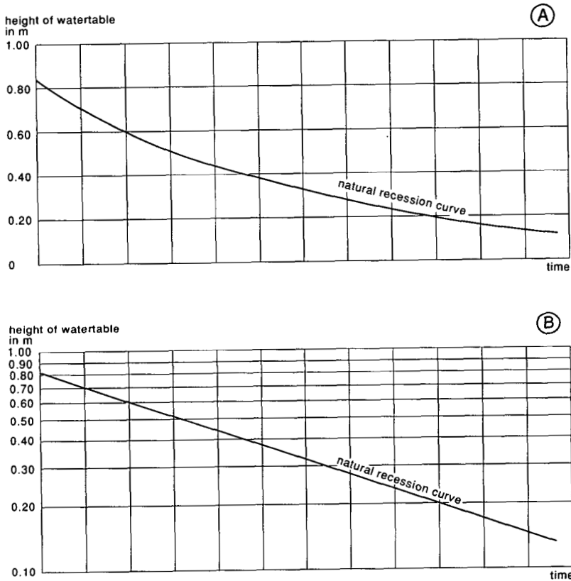
Figure 2.20 Natural recession of groundwater level: A: Linear scale; B: Logarithmic scale
