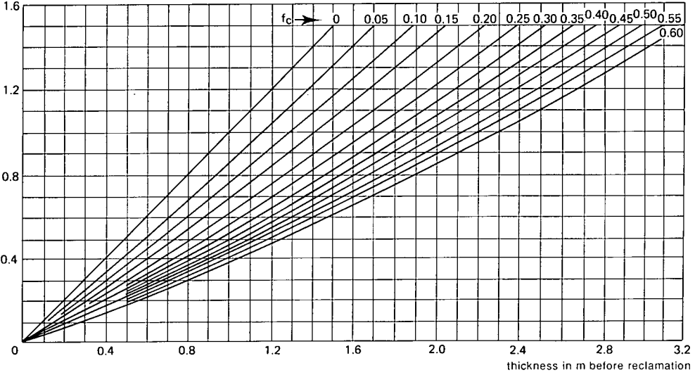
Figure 13.13 Relationship between the initial and final thickness of sediments with different clay contents f_c in the IJsselmeerpolders (De Gloopper 1973)
