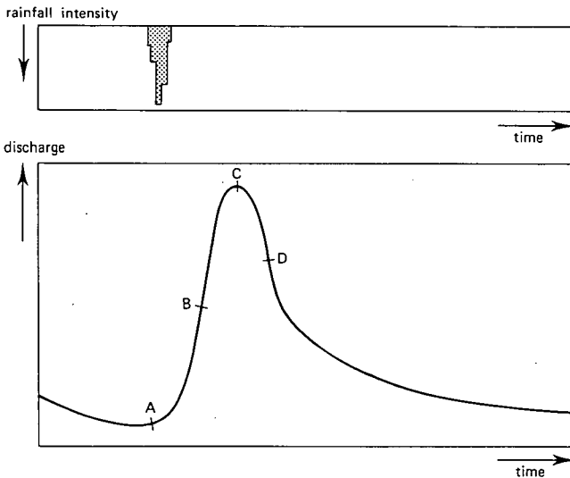
Figure 4.6 A single-peaked hydrograph of total runoff
