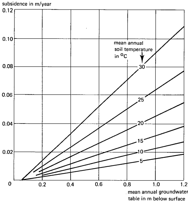
Figure 13.15 The relationship between the annual subsidence rate in the layer above the watertable and the mean annual watertable for different soil temperatures ( ^{\circ}\text{C} at 0.10 m below surface)
