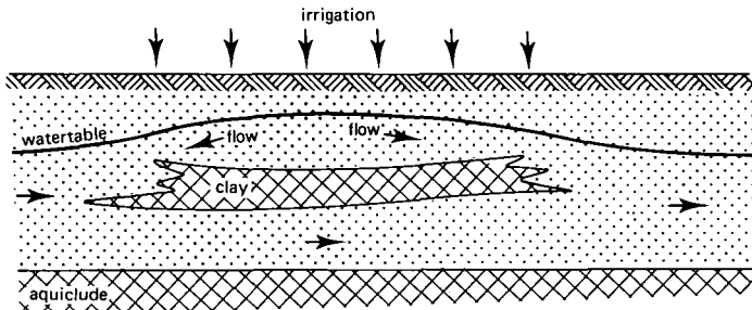
Figure 2.34 A clay lens under an irrigated area impedes the downward flow of excess irrigation water
