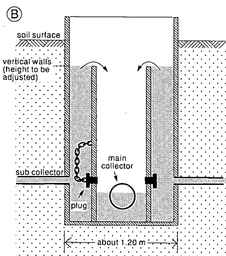
Figure 21.8 Prototype of a closing device in a manhole A: Top view B: Section A-A
