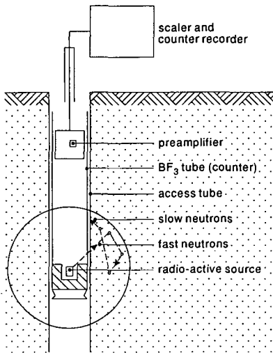
Figure 11.1 Neutron probe to measure soil-water content
