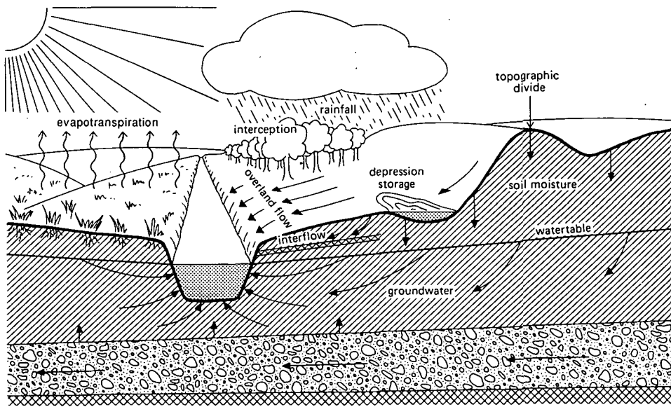
Figure 4.4 Schematization of the runoff cycle
