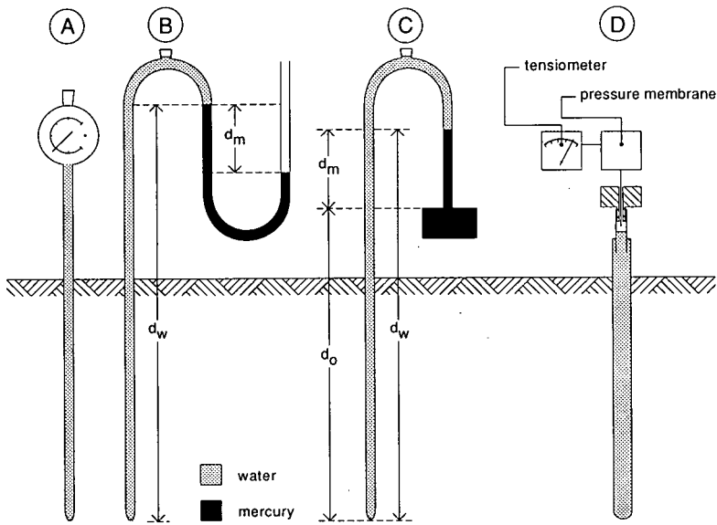
Figure 11.7 Tensiometers
