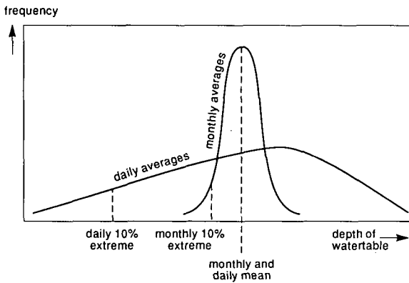
Figure 17.6 Frequency distributions of daily average and monthly average depths of the watertable
