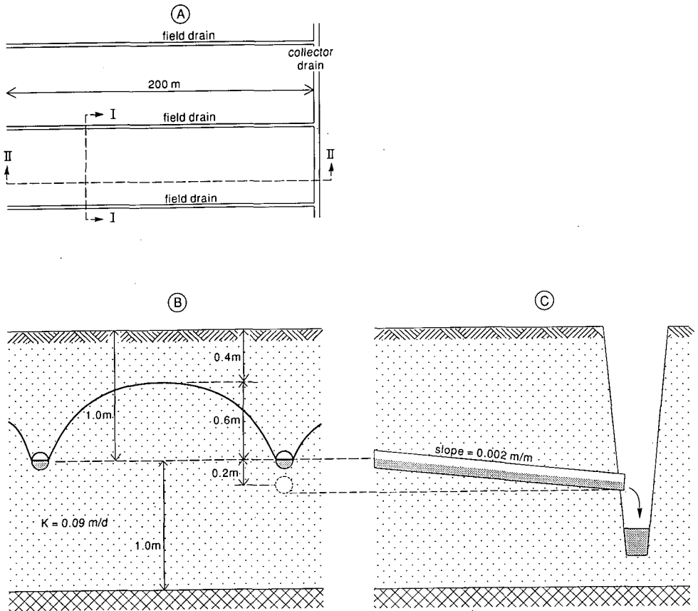
Figure 21.49 Example of subsurface drainage system used to describe malfunctioning of the system
