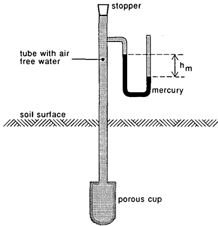
Figure 3.5 A tensiometer
