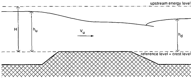
Figure 24.20 Subcritical flow over a weir
